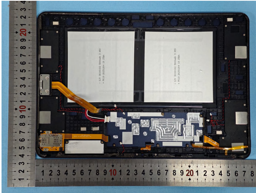
Photo 11 Internal photos of EUT Model: AF12/ES418
