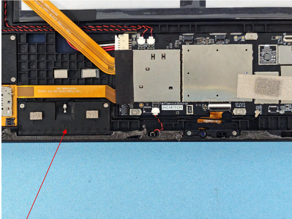
Photo 3 Internal photos of EUT Model: AF12/ES418
