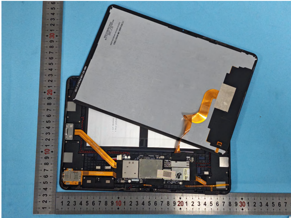
Photo 1 Internal photos of EUT Model: AF12/ES418
