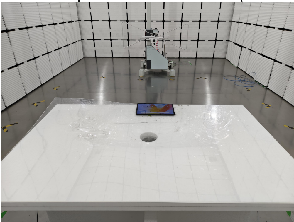
Photo 1 Test Setup Photos of Radiated Emission Test (30-1000MHz)
