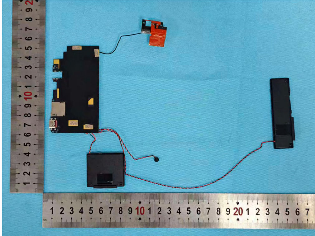
Photo 5 Internal photos of EUT Main Test Model: ES316B/B11AIR
