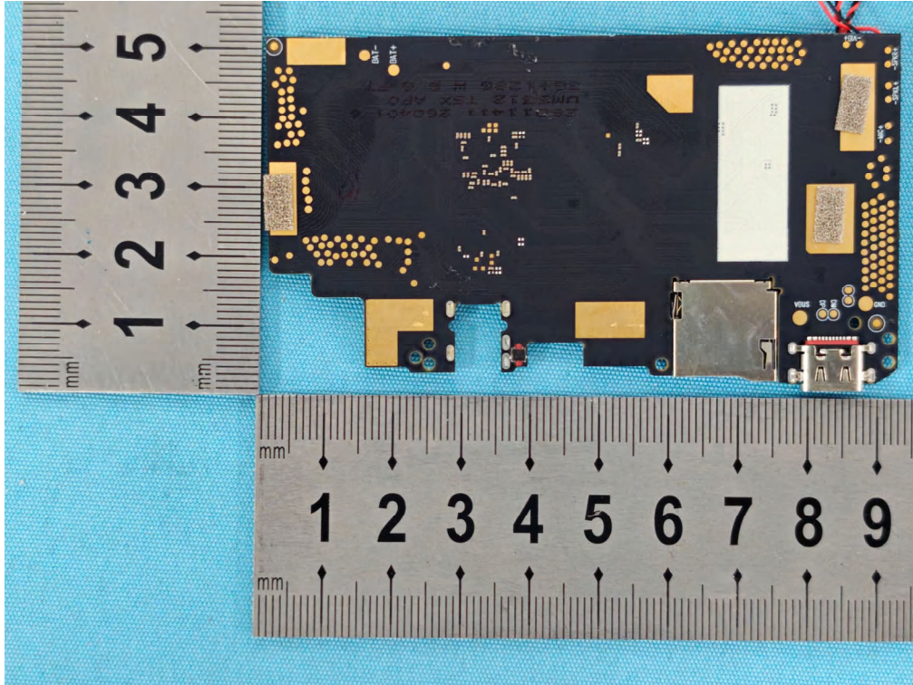
Photo 9 Internal photos of EUT Main Test Model: ES316B/B11AIR
