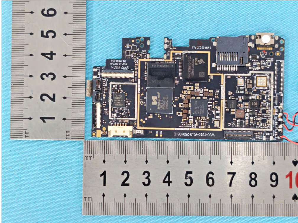
Photo 7 Internal photos of EUT Main Test Model: ES316B/B11AIR
