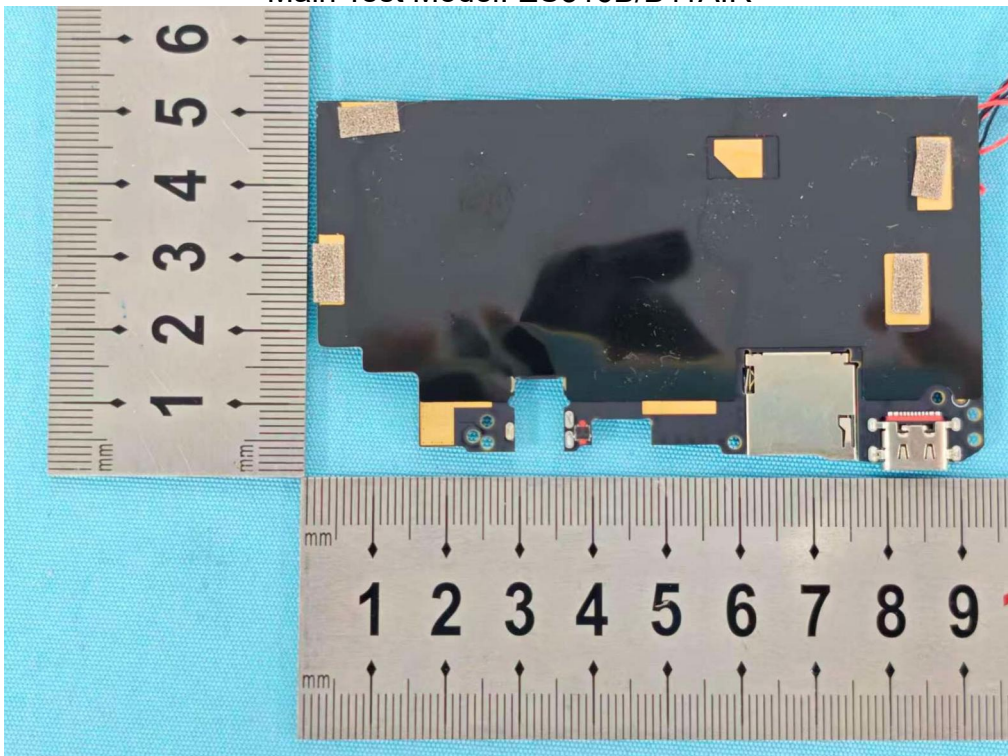
Photo 8 Internal photos of EUT Main Test Model: ES316B/B11AIR
