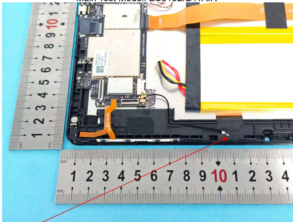
Photo 3 Internal photos of EUT Main Test Model: ES316B/B11AIR
