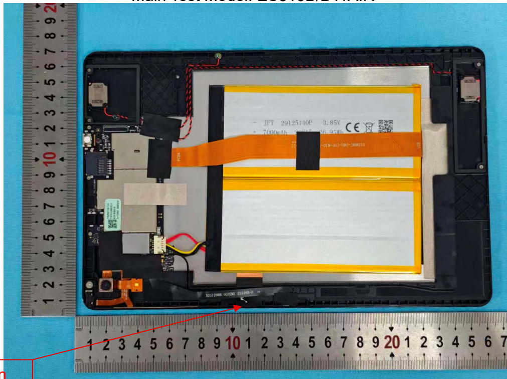
Photo 2 Internal photos of EUT Main Test Model: ES316B/B11AIR
