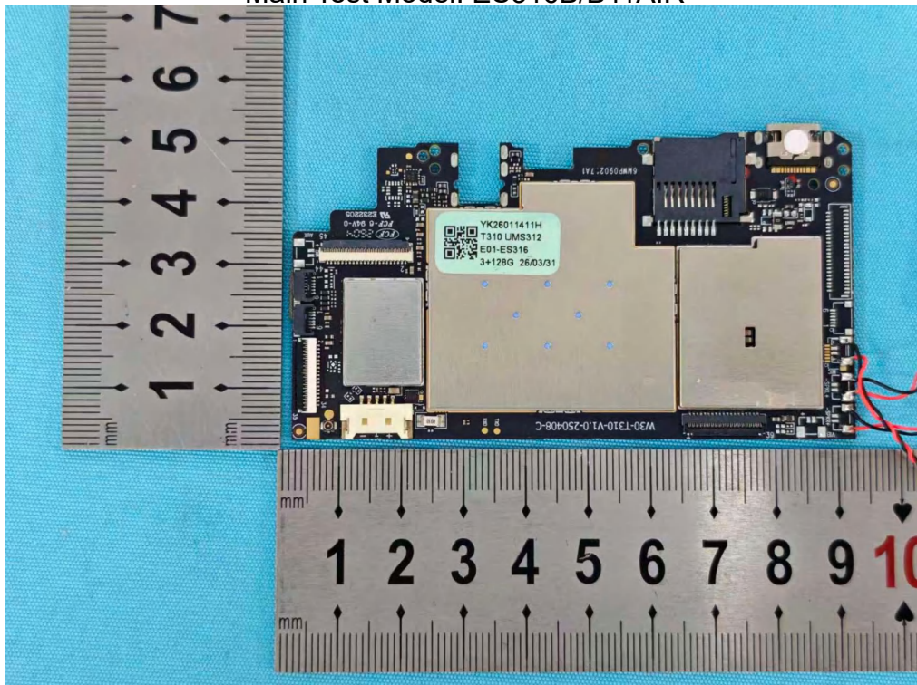
Photo 6 Internal photos of EUT Main Test Model: ES316B/B11AIR
