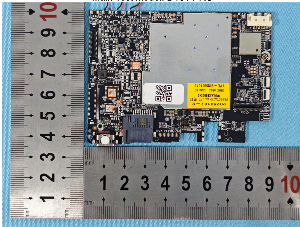
Photo 4 Internal photos of EUT Main Test Model: D101 PRO
