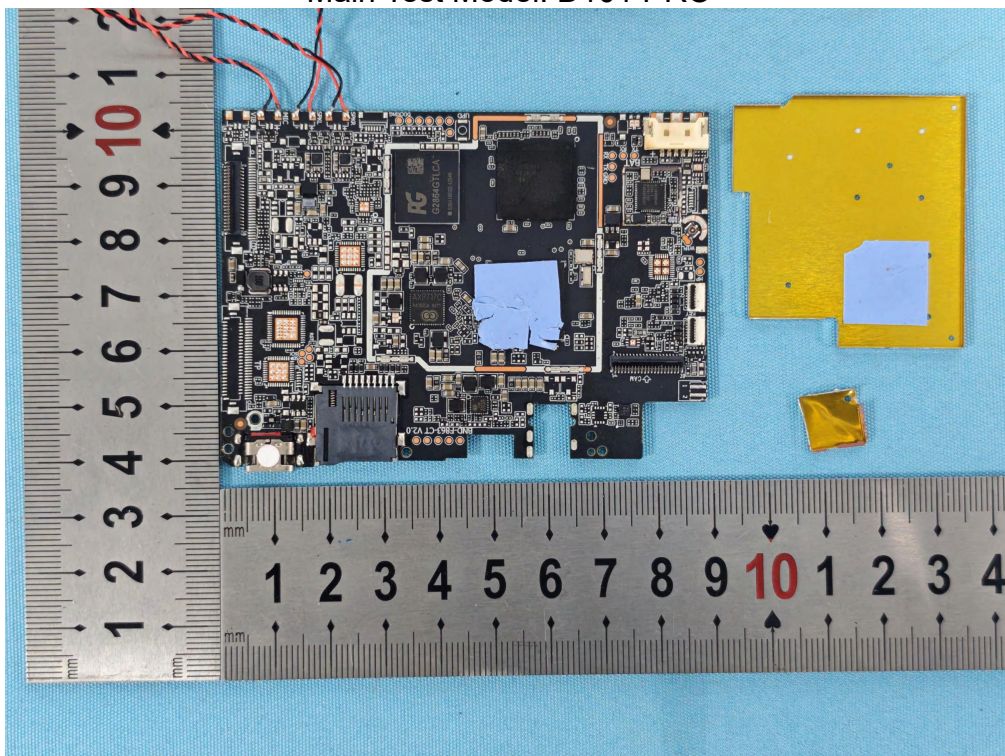
Photo 6 Internal photos of EUT Main Test Model: D101 PRO
