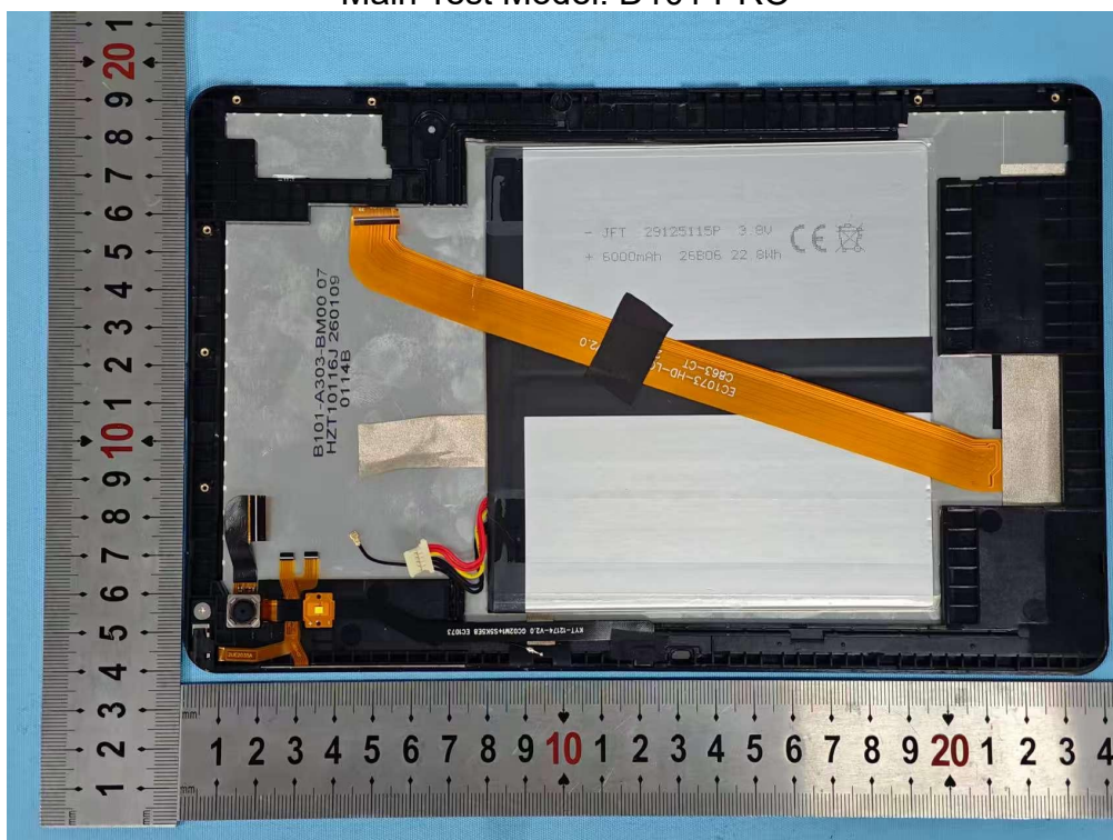
Photo 10 Internal photos of EUT Main Test Model: D101 PRO
