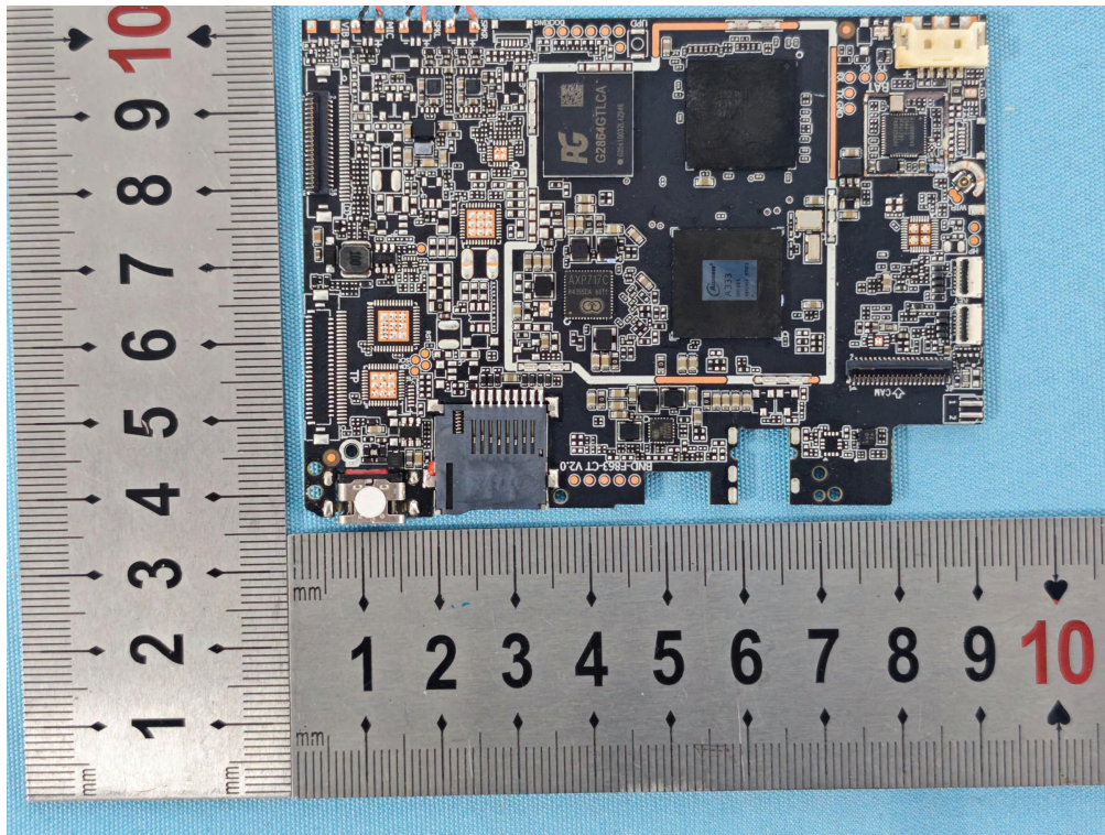
Photo 7 Internal photos of EUT Main Test Model: D101 PRO
