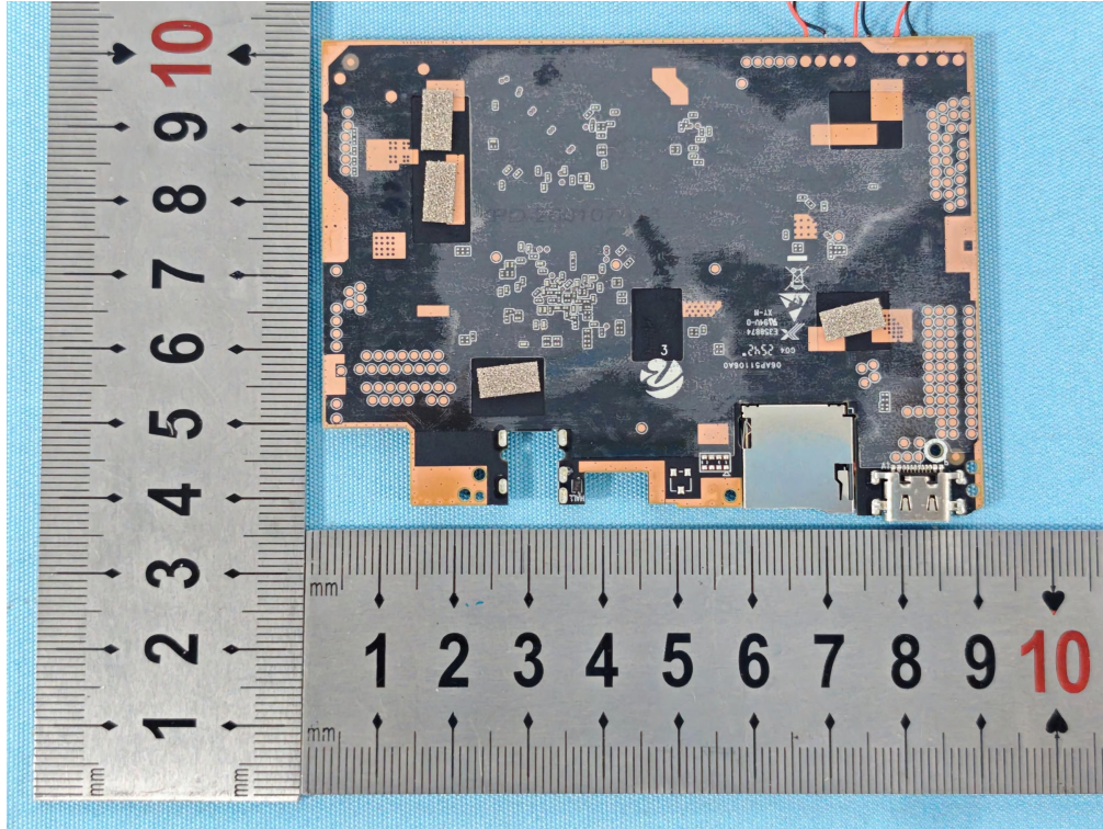
Photo 5 Internal photos of EUT Main Test Model: D101 PRO
