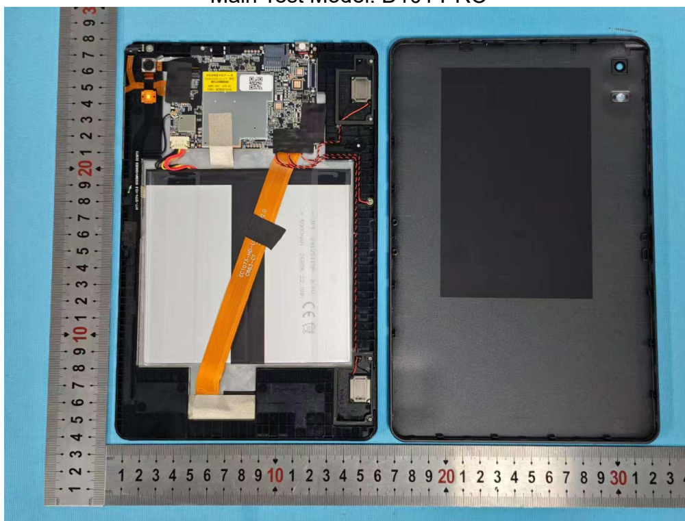
Photo 1 Internal photos of EUT Main Test Model: D101 PRO
