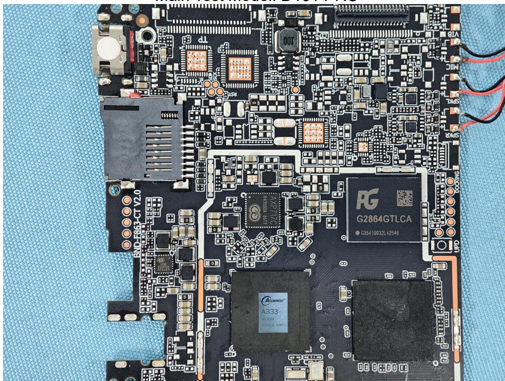
Photo 8 Internal photos of EUT Main Test Model: D101 PRO
