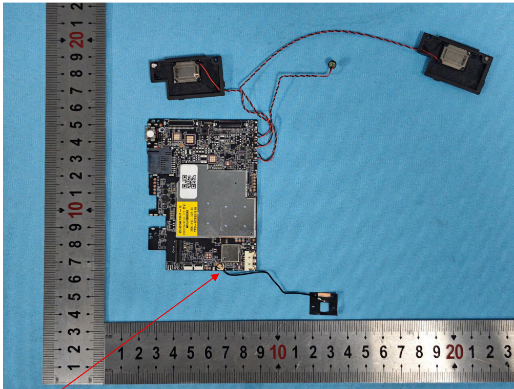
Photo 3 Internal photos of EUT Main Test Model: D101 PRO
