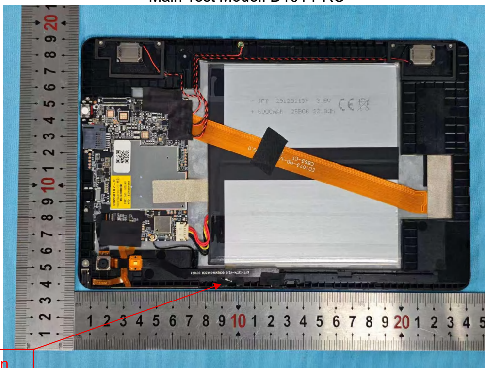
Photo 2 Internal photos of EUT Main Test Model: D101 PRO
