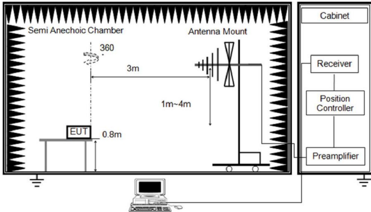
(B) Radiated Emission Test Set-Up, Frequency below 1000MHz Below 1 GHz and above 30 MHz
