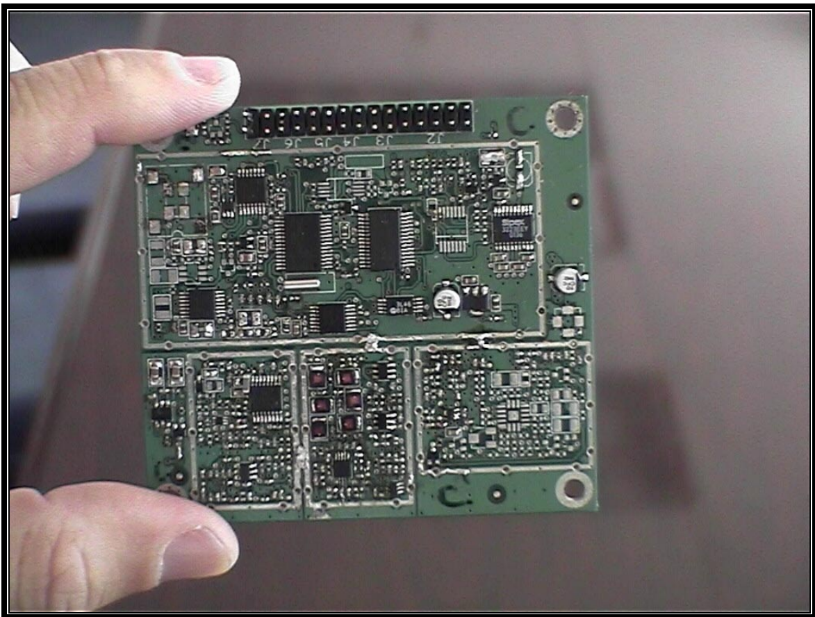
Photograph 2: Top side of module – shields removed
