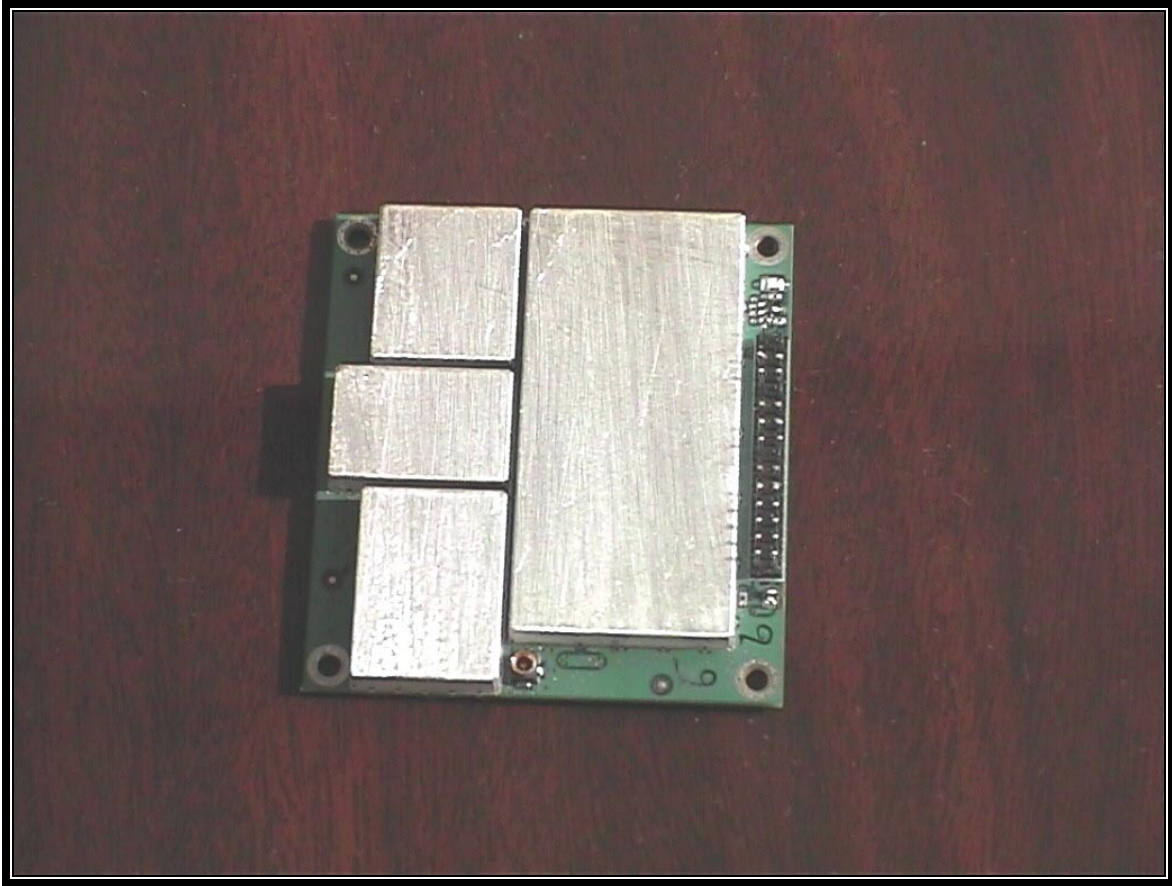
Photograph 1: Top side of module – with shields
