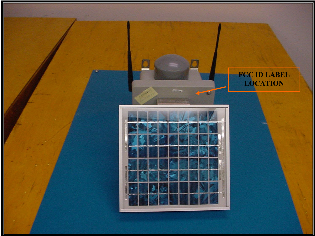
PHOTOGRAPH 1: FCC ID LABEL LOCATION ON FRONT OF EUT
