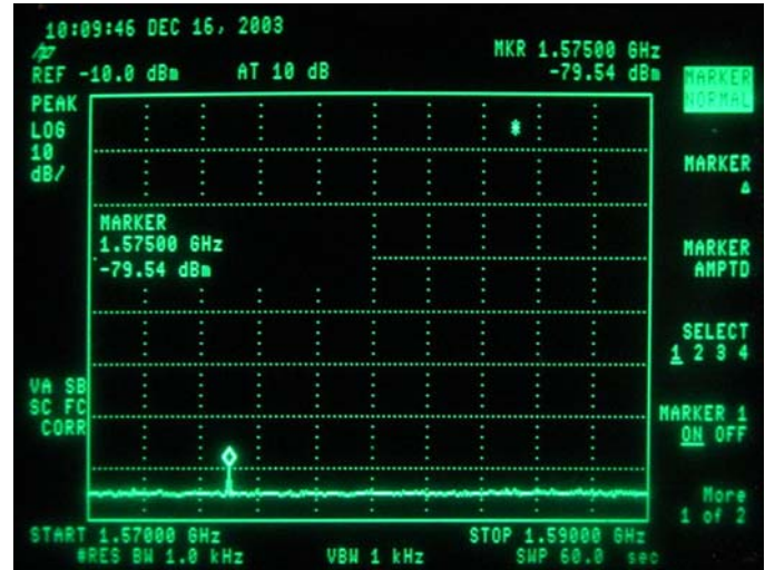
FIG 2: Frequency Span 1570 – 1590 MHz.
