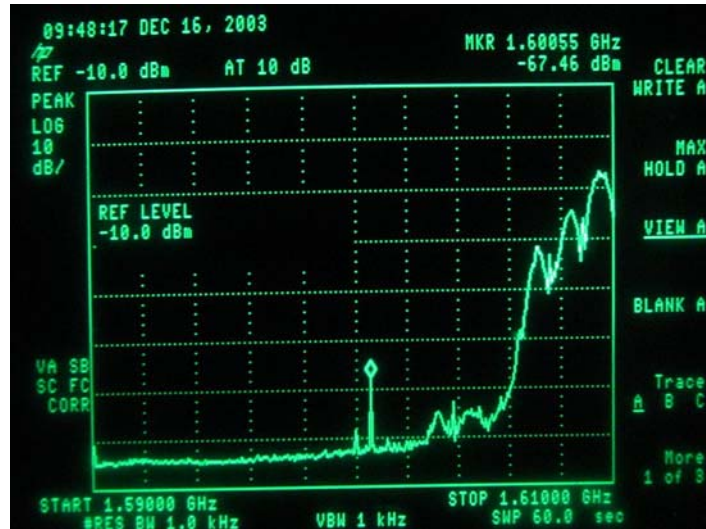
FIG 3: Frequency Span 1590 – 1610 MHz.
