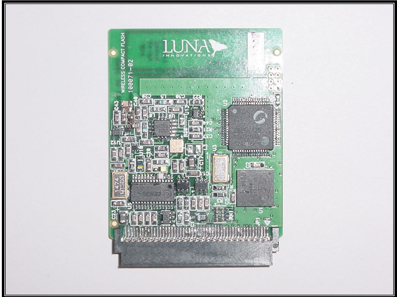
PHOTOGRAPH 5: iCFR FRONT
