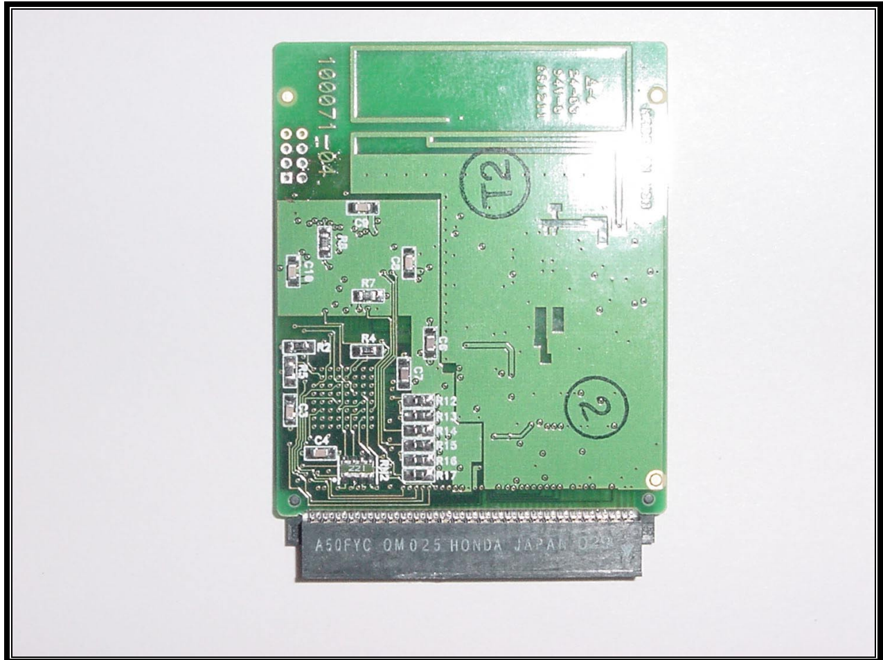
PHOTOGRAPH 6: iCFR REAR
