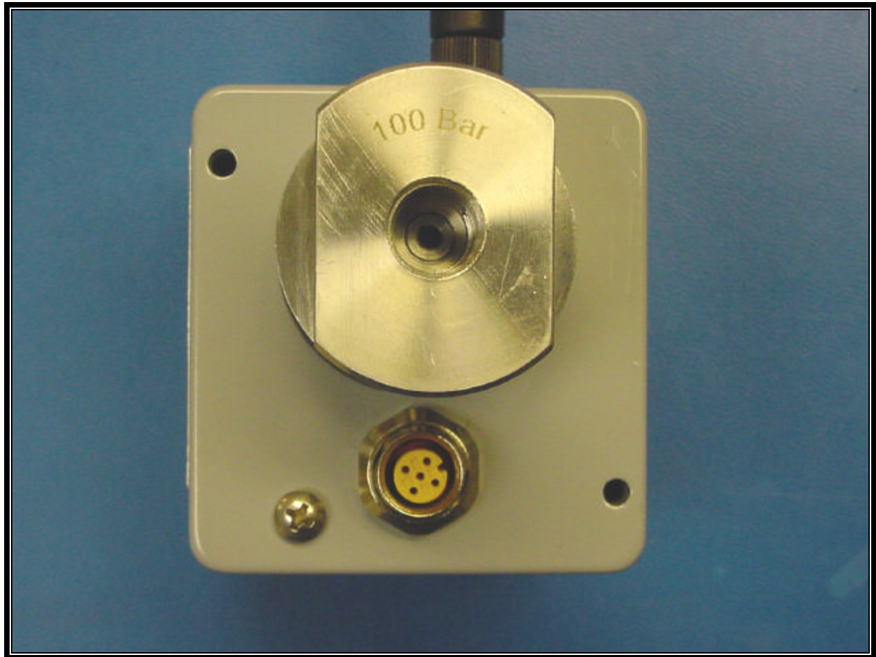
PHOTOGRAPH 22: iWPM-T BOTTOM
