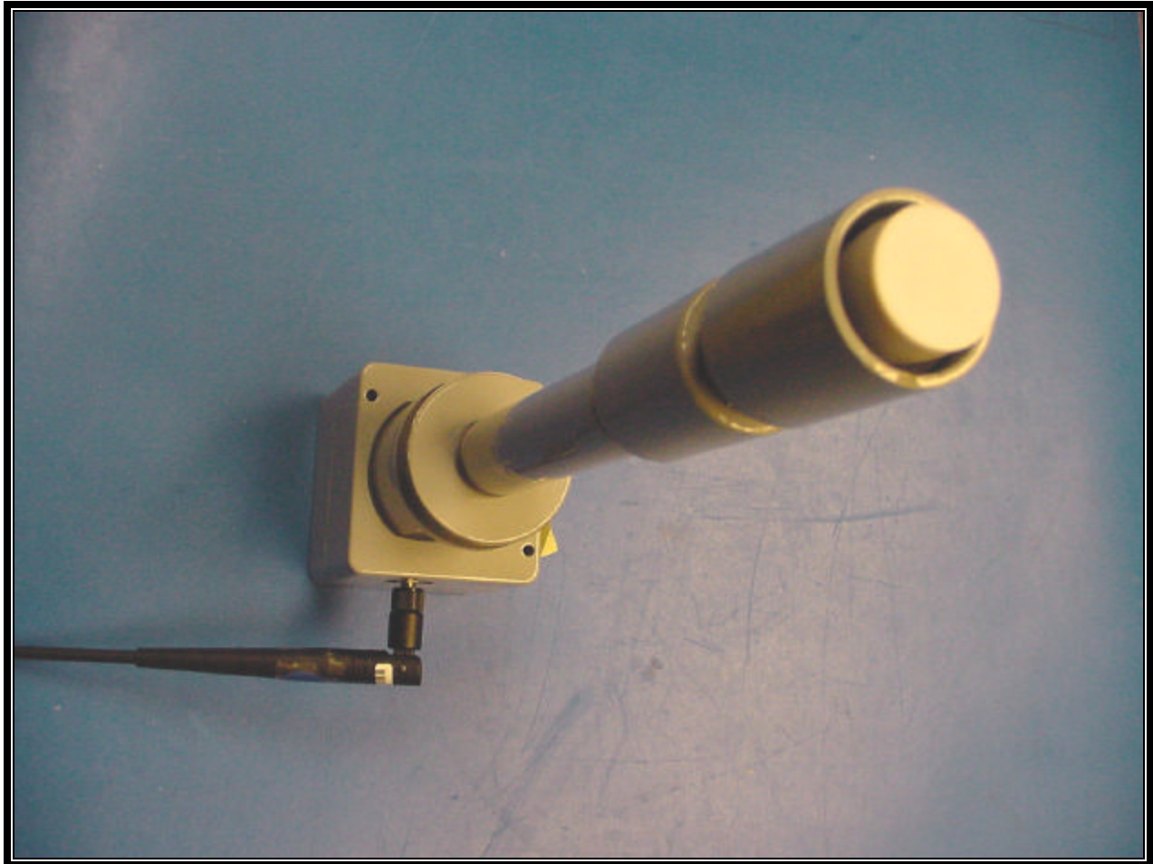
PHOTOGRAPH 17: iTLM-1 BOTTOM
