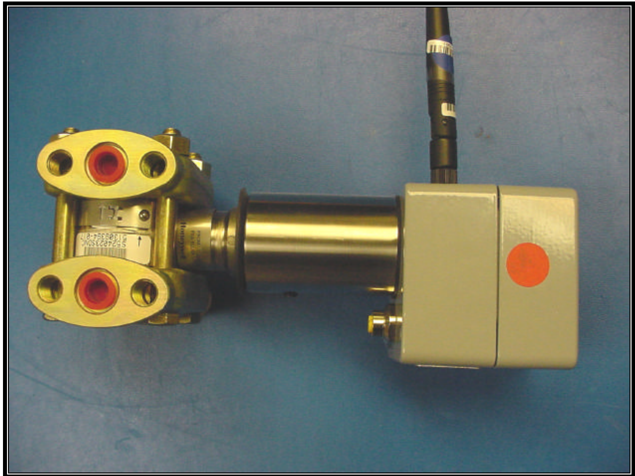
PHOTOGRAPH 14: iEFM SIDE
