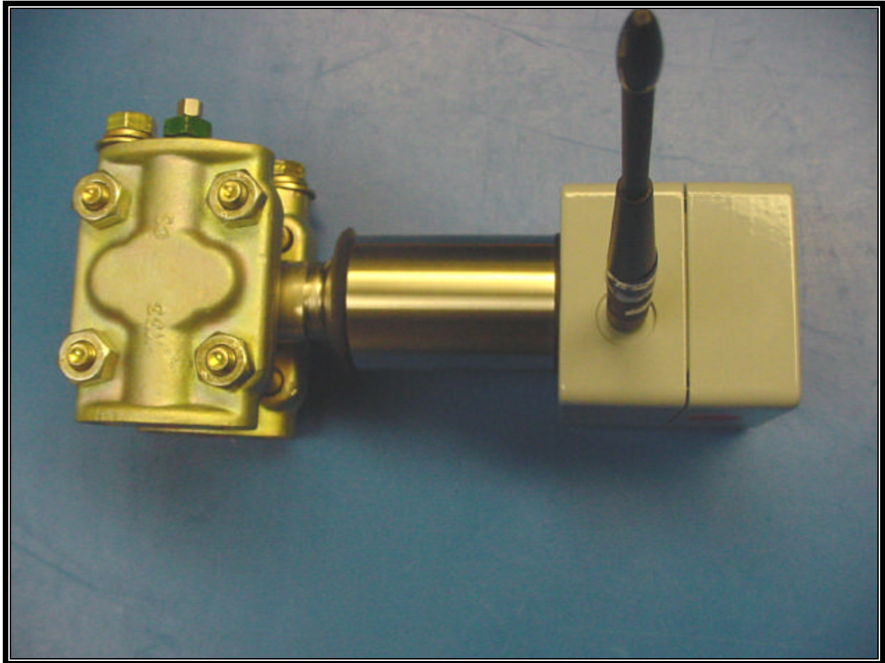
PHOTOGRAPH 15: iEFM SIDE
