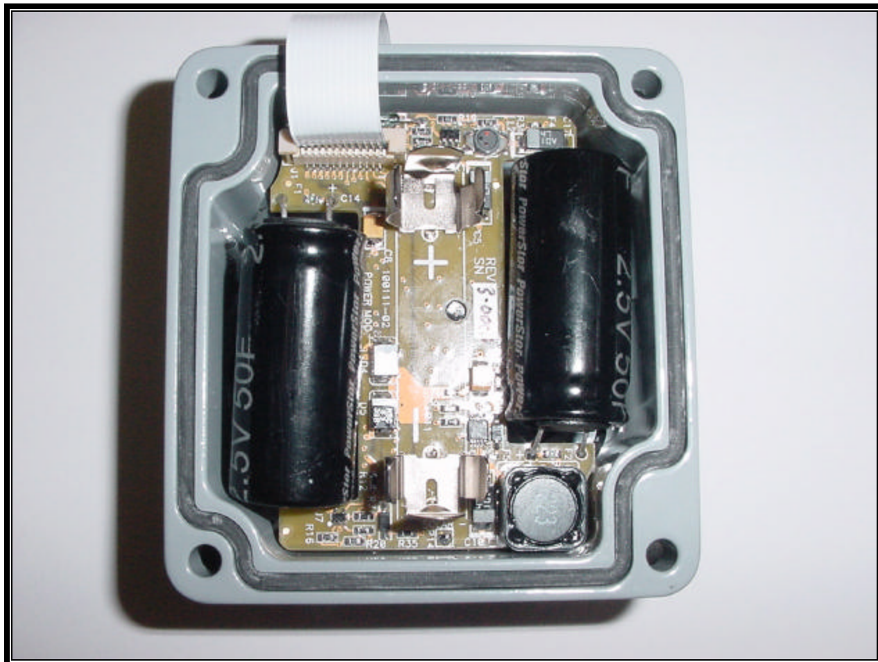
PHOTOGRAPH 29: SOLAR CELL AND BATTERY CIRCUITRY (FRONT)
