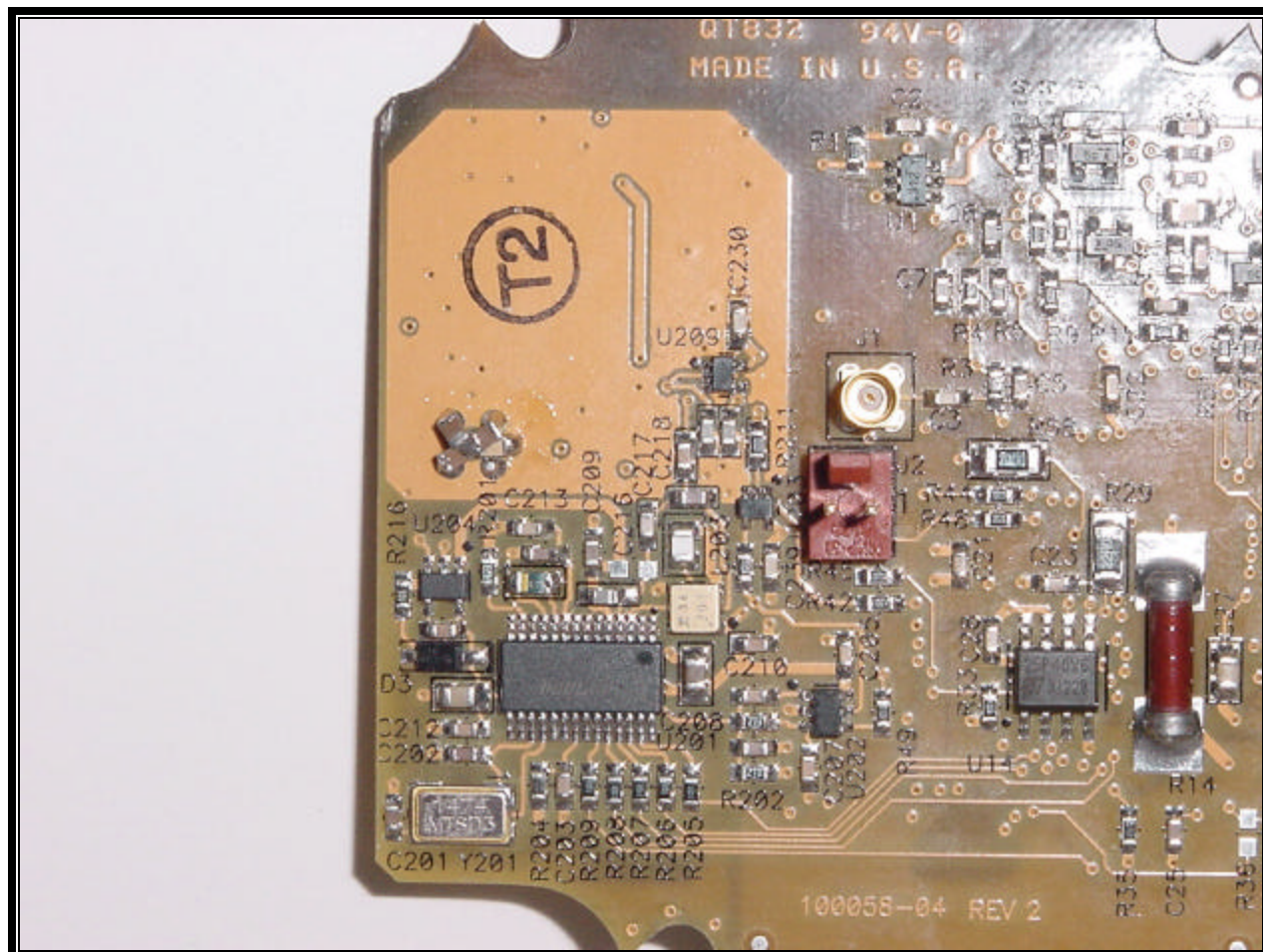
PHOTOGRAPH 32: iTLM-1 RF SECTION BOTTOM CLOSE-UP
