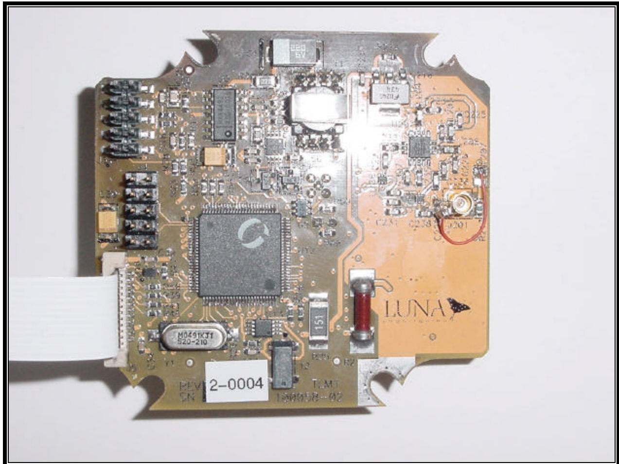
PHOTOGRAPH 33: iTLM-1 TOP
