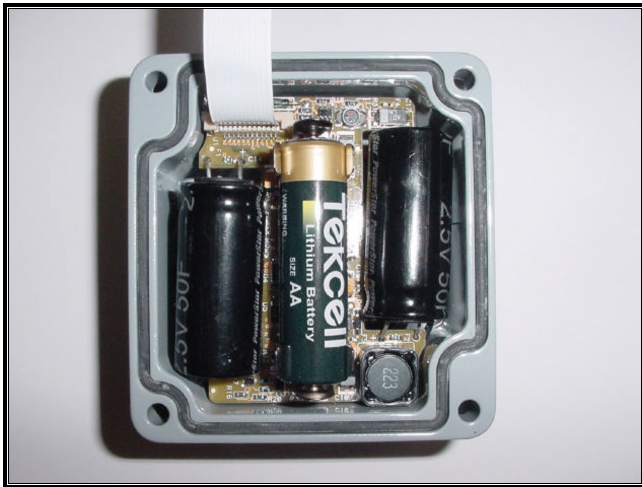
PHOTOGRAPH 28: SOLAR CELL AND BATTERY CIRCUITRY (FRONT)
