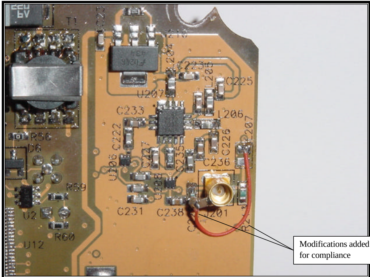
PHOTOGRAPH 31: iTLM-1 RF SECTION TOP CLOSE-UP
