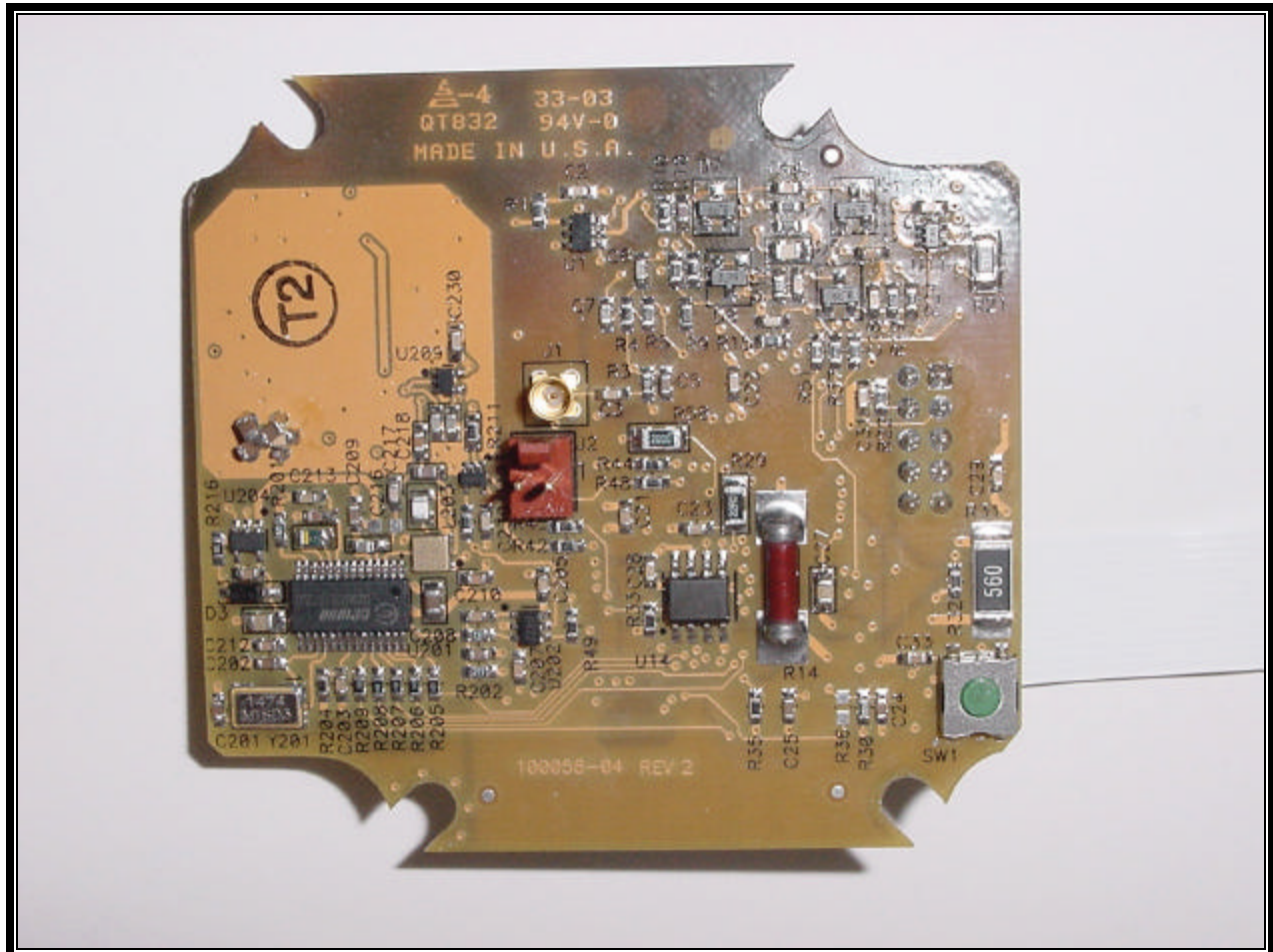
PHOTOGRAPH 34: iTLM-1 BOTTOM
