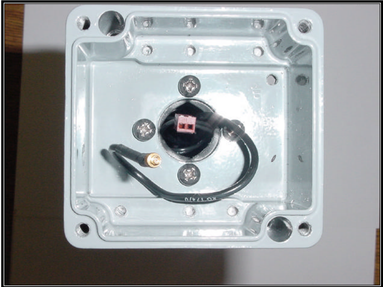
PHOTOGRAPH 35: iTLM-1 ENCLOSURE
