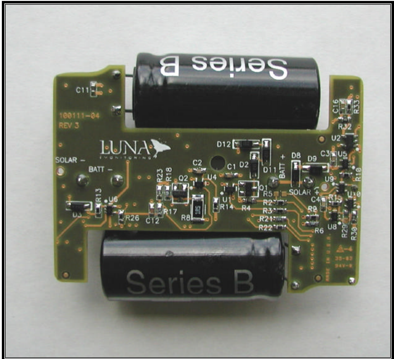
PHOTOGRAPH 30: SOLAR CELL AND BATTERY CIRCUITRY (BACK)
