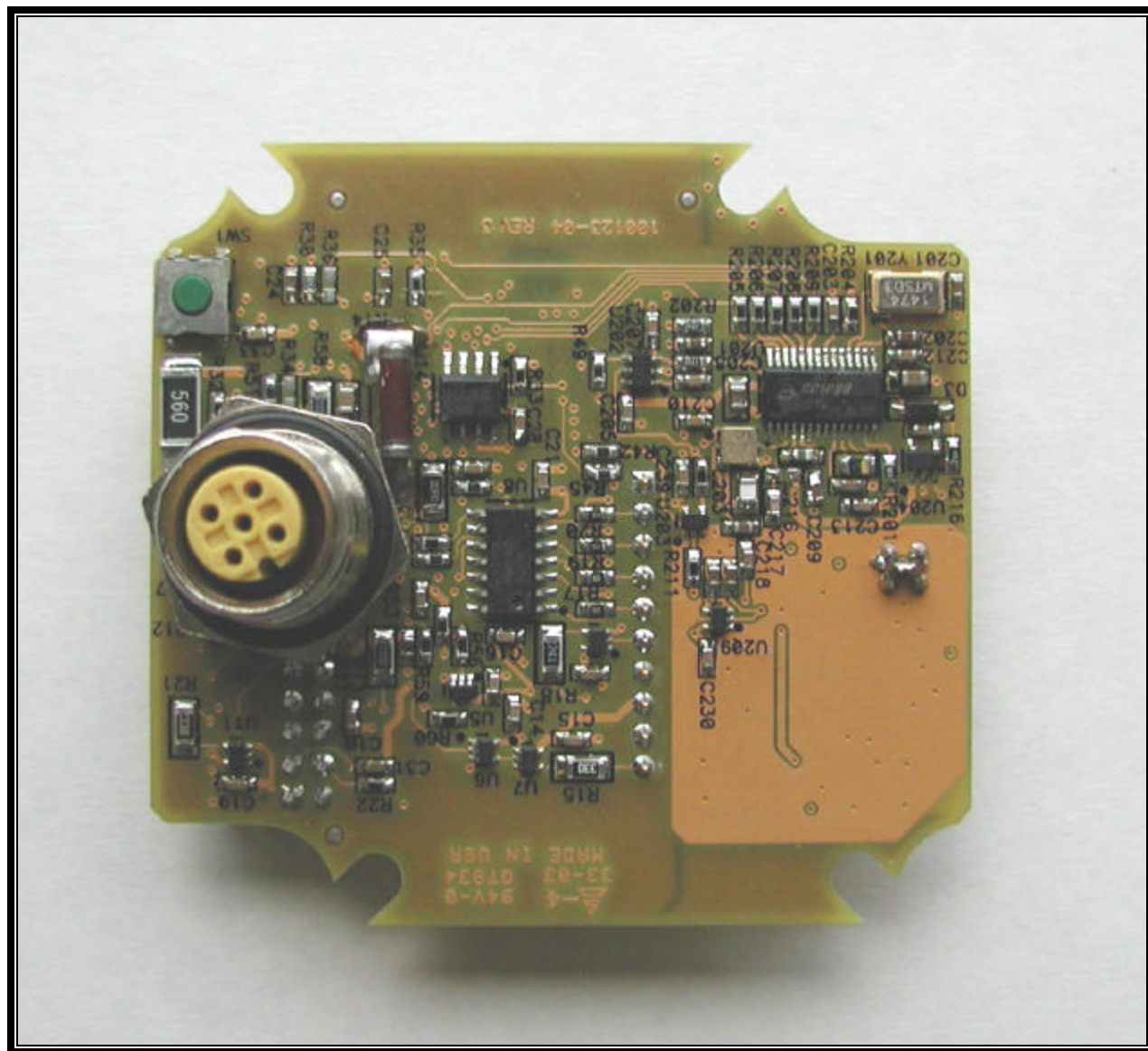
PHOTOGRAPH 37: iEFM (BACK)
