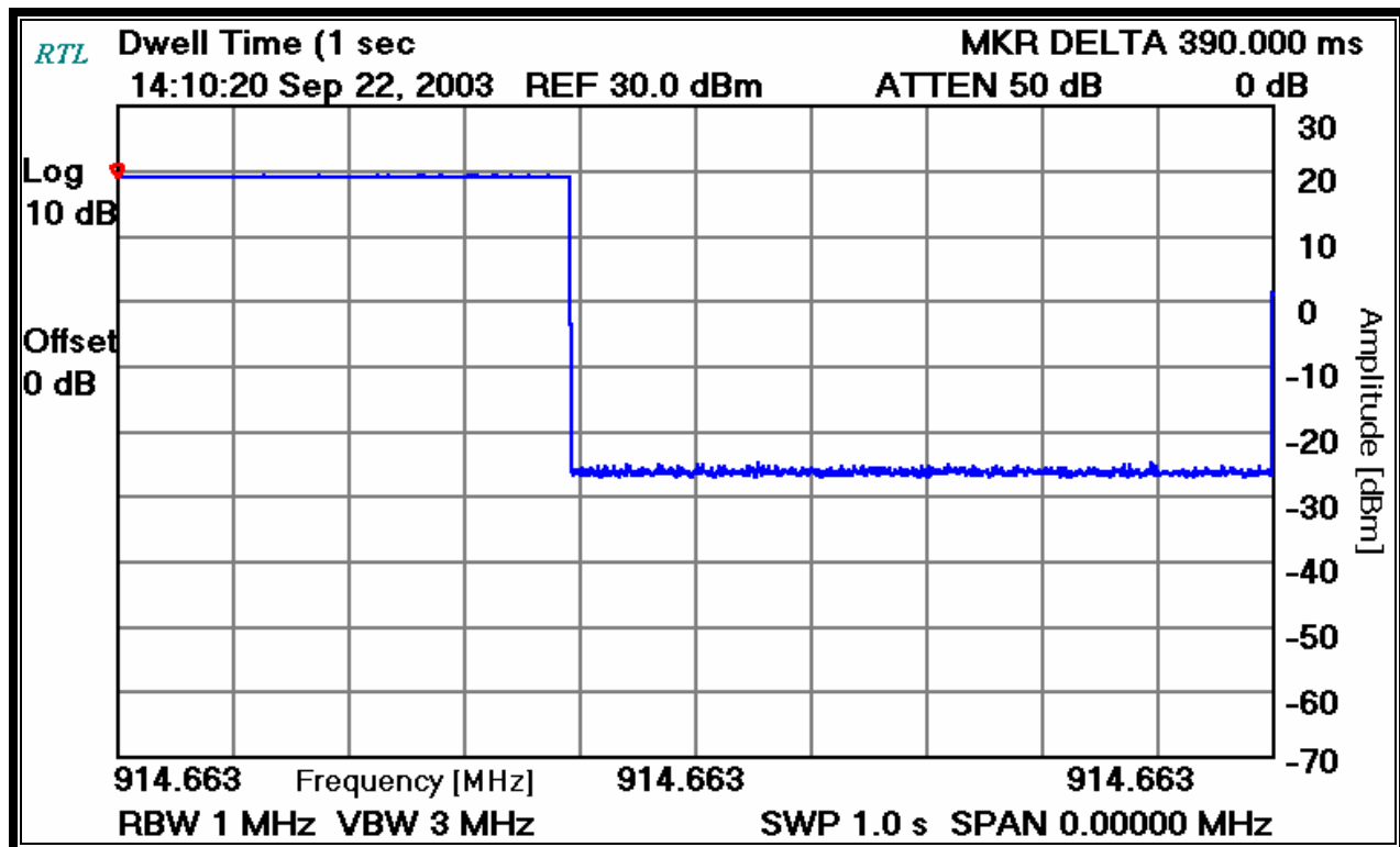
PLOT 11-2: TIME OF OCCUPANCY (DWELL TIME)
