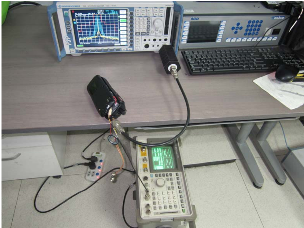
Test setup photos of the EUT
