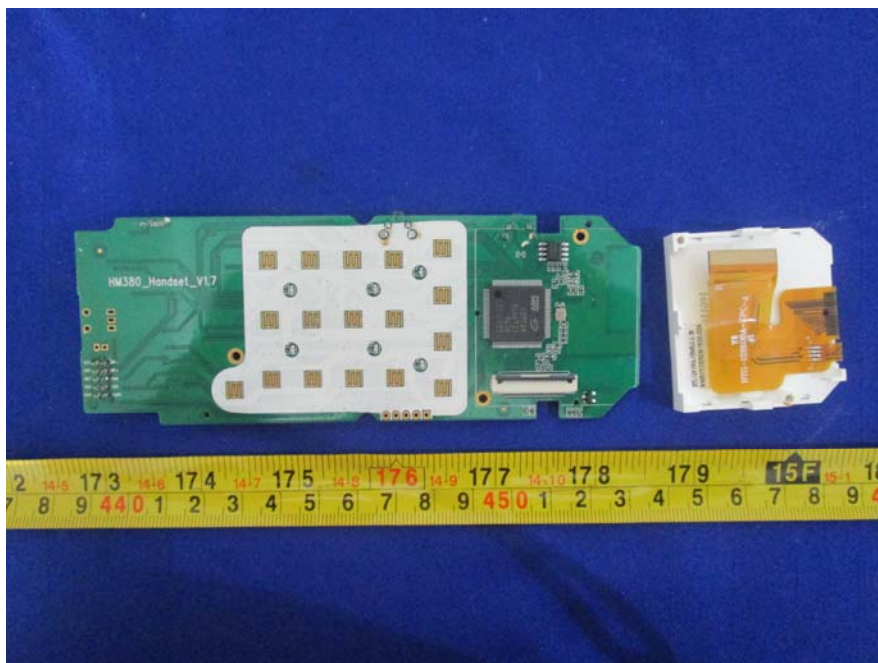
EUT –MIC Uncover View
