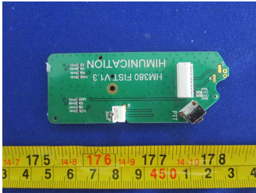
EUT – Small MIC Mainboard Bottom View
