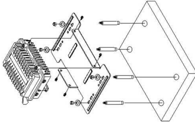
Wall Mounting Figure
