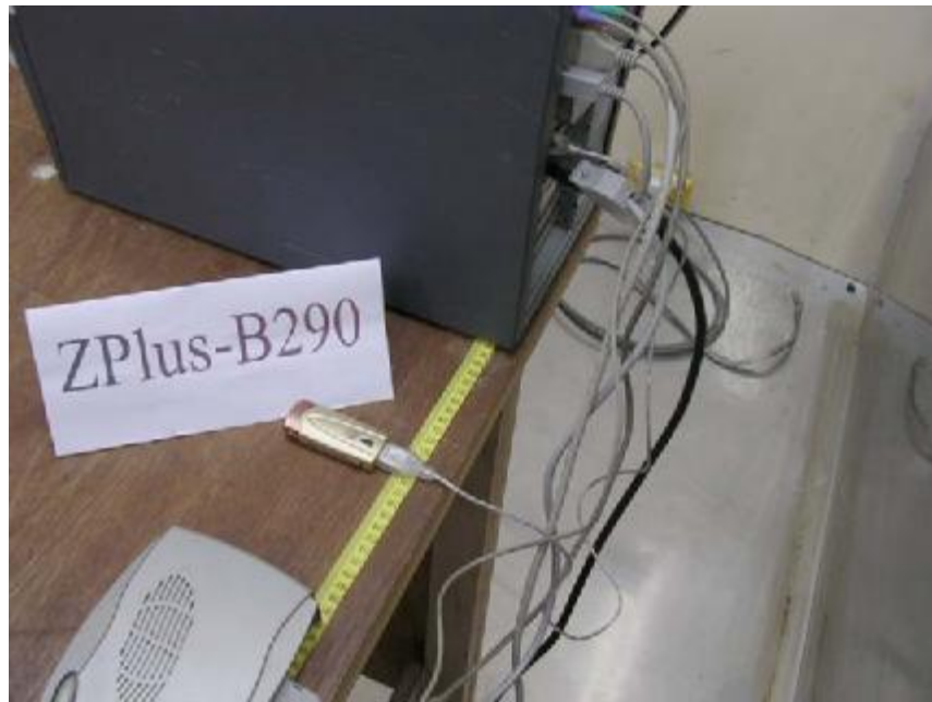
Photo 3: Conducted Test set-up
