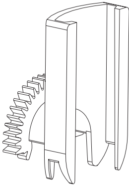
Figure 8: Antenna Shroud
