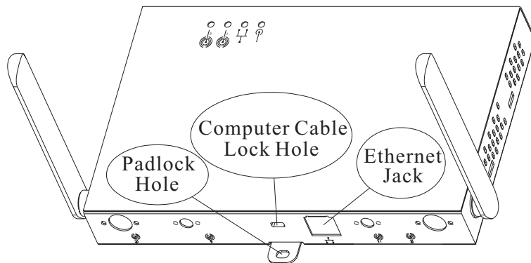
Figure 1: Rear View Of Altitude 300-2i™
