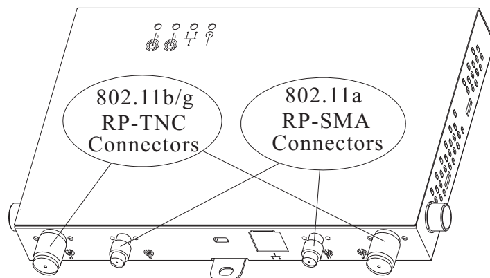
Figure 2: Rear View Of Altitude 300-2d™
