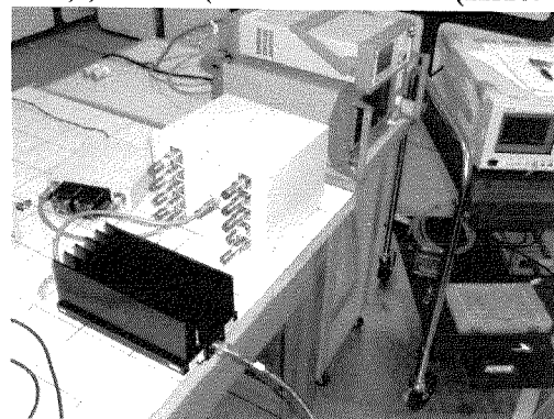
( With Combiner(HX69-C) )
