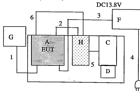
With Combiner(HX69-V)
