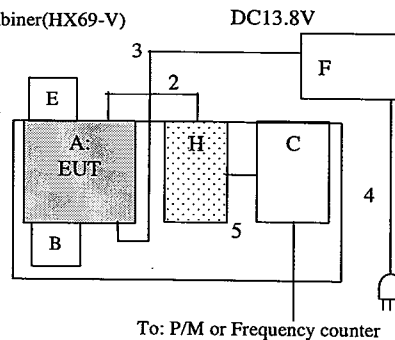
With Combiner(HX69-V)
