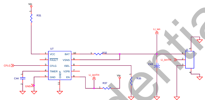
CHARGE CIRCUIT
