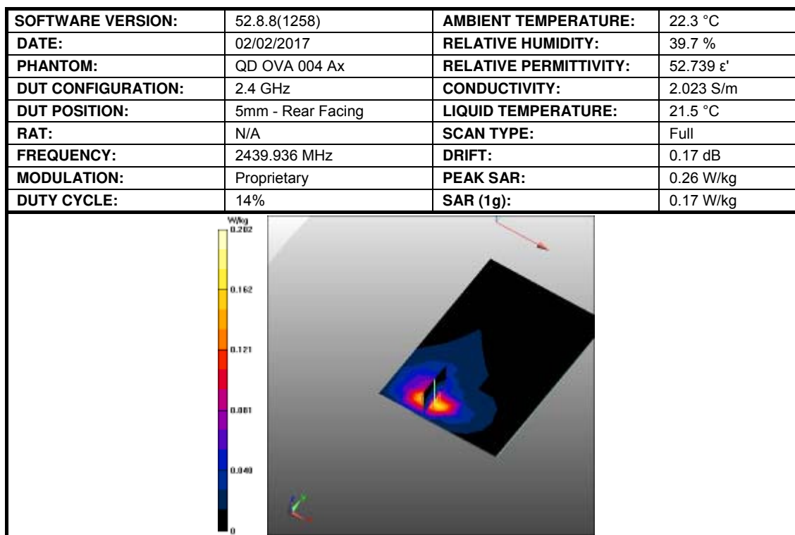
Figure 4: SAR Body Testing Results for the IML Connector 2436.936 MHz.
