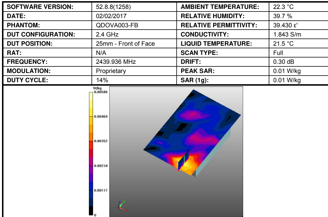
Figure 2: SAR Body Testing Results for the IML Connector at 2436.936 MHz
