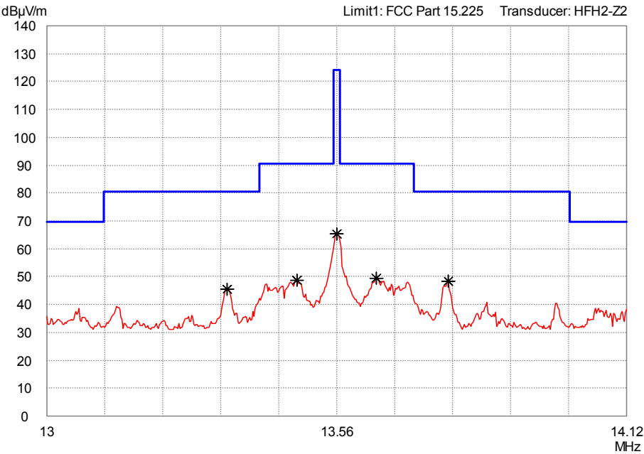
Figure 1: RBW = 10 kHz
