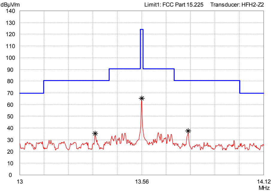
Figure 2: RBW = 1 kHz
