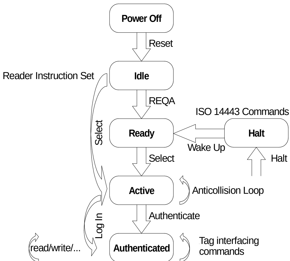
Figure 5-4: State diagram
