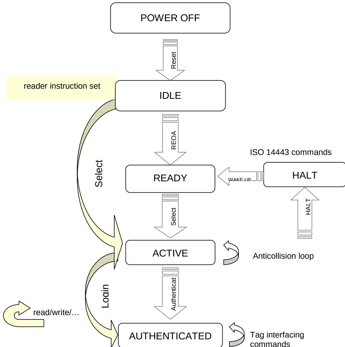
Figure 5-1: State diagram
