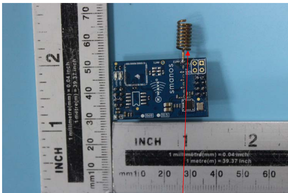
Antenna(915MHz RX)
