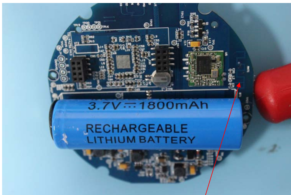
Antenna(WIFI)
