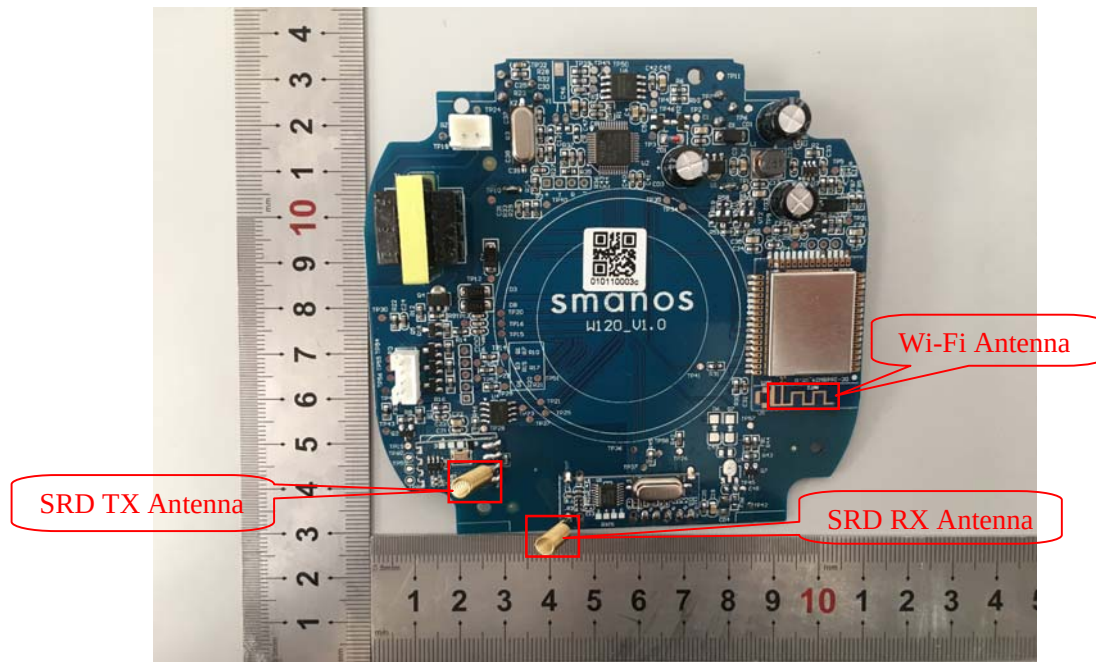
EUT – PCB Top View
