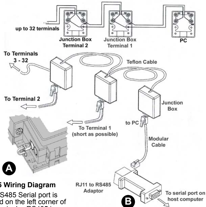
Junction Box "Daisy Chain" Wiring Diagram
