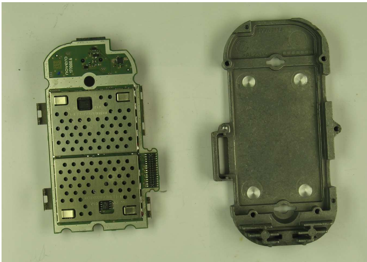
Bottom view main PCB with shielding
