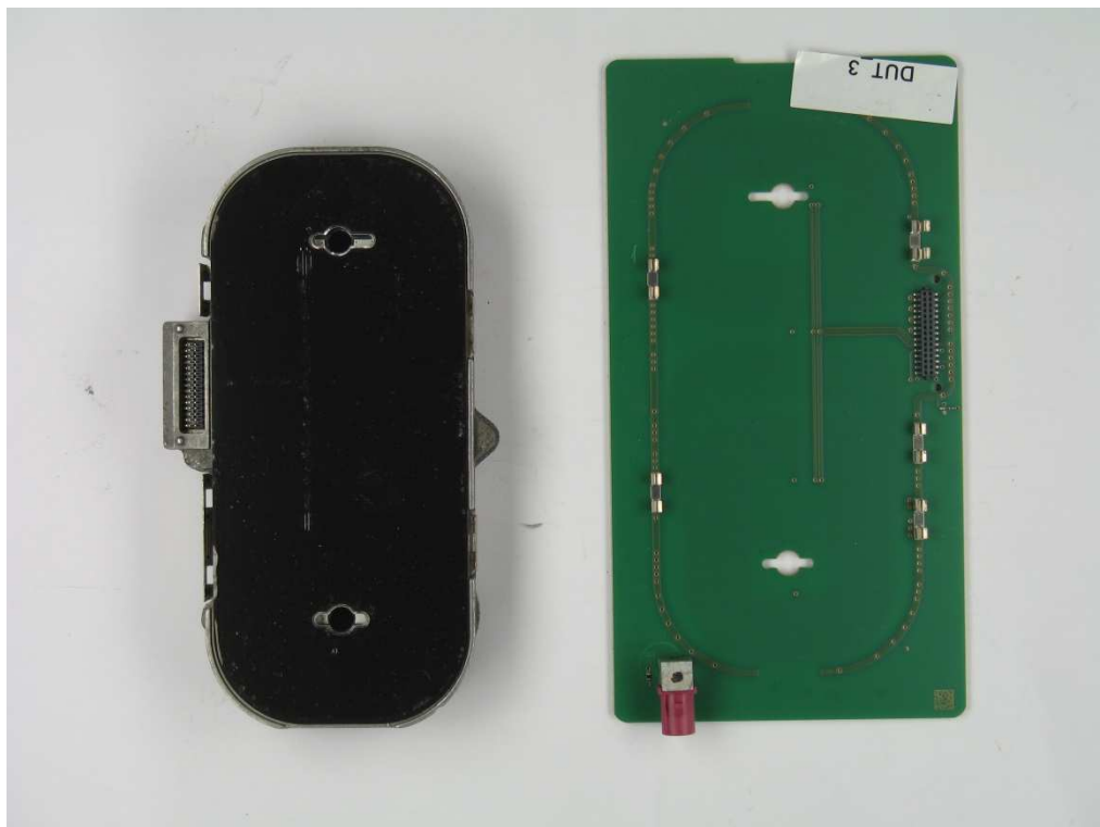
Top view coil board with antenna connector
