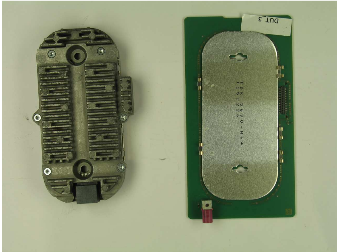
Inside view with cooling element and ferrite plate
