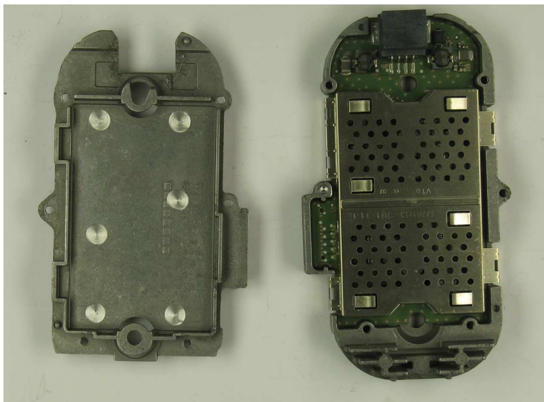
Top view main PCB with shielding
