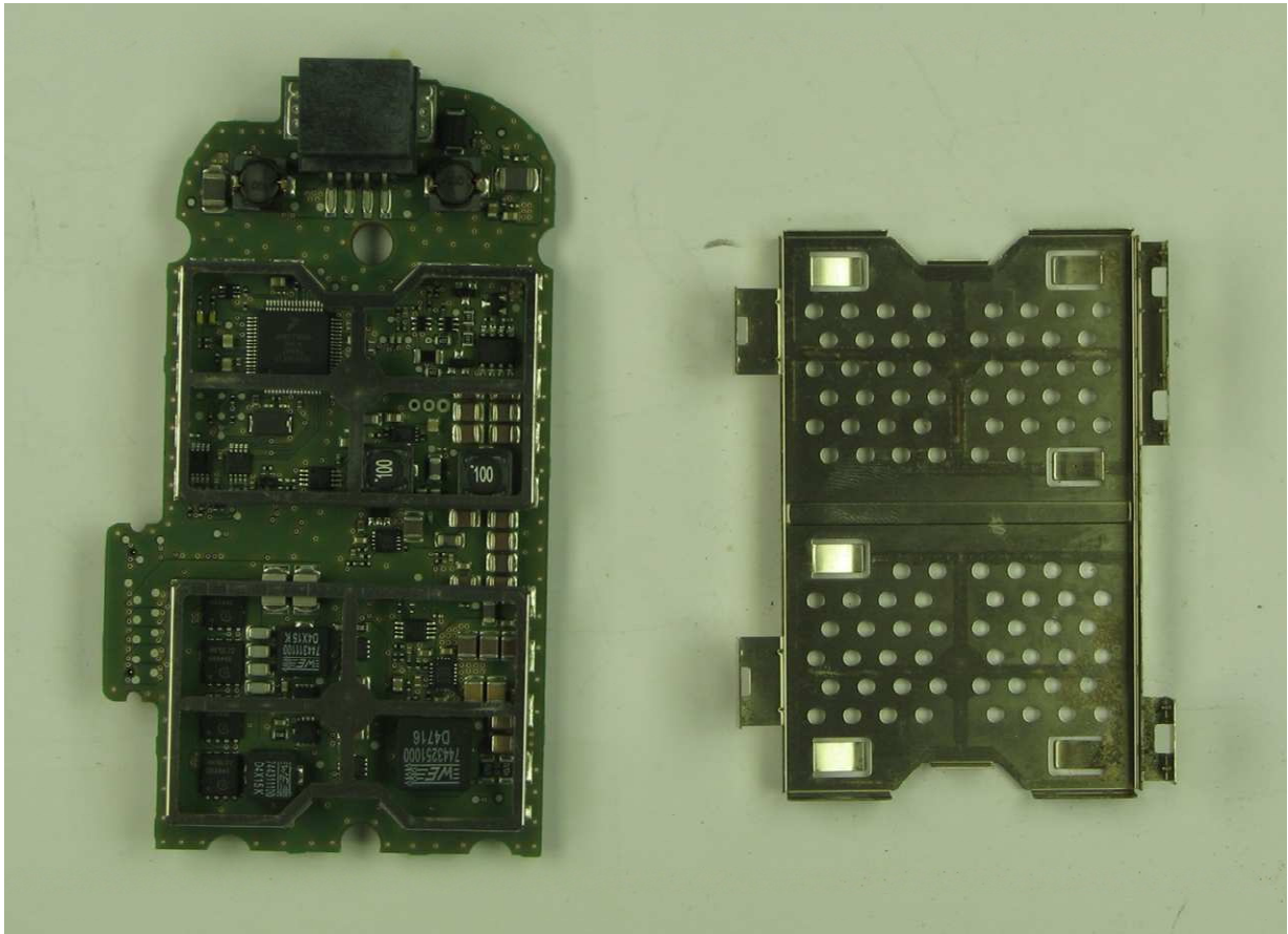
Top view main PCB without shielding
