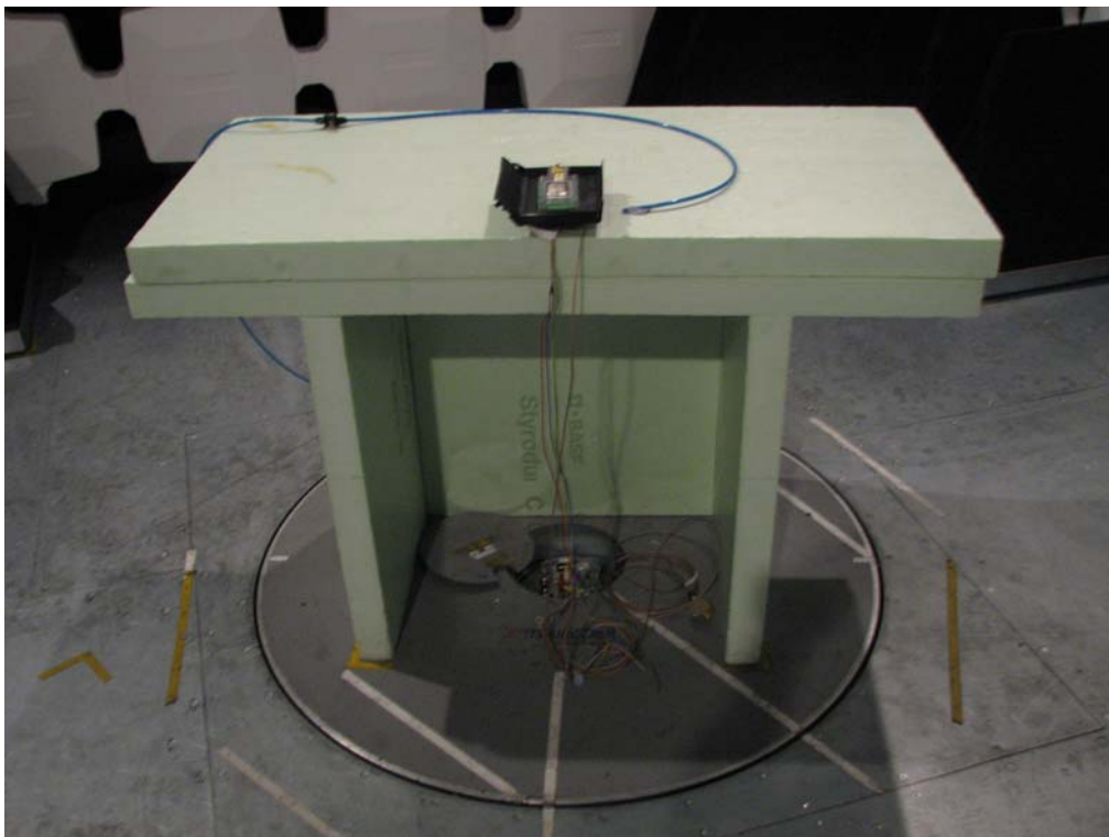
FCC Part 15C Radiated Emissions Test Setup 30-1000MHz
