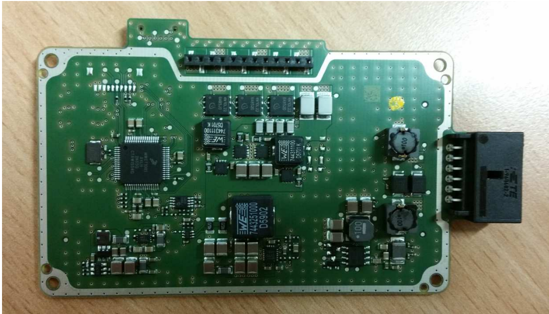
Top View Main board
