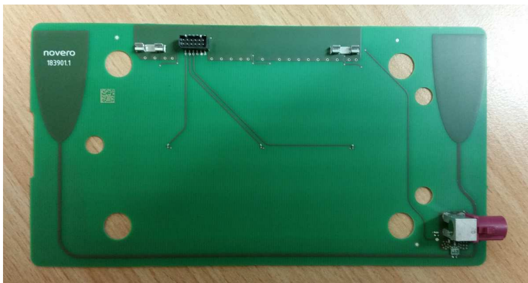
Top view antenna board with Fakra antenna connector
