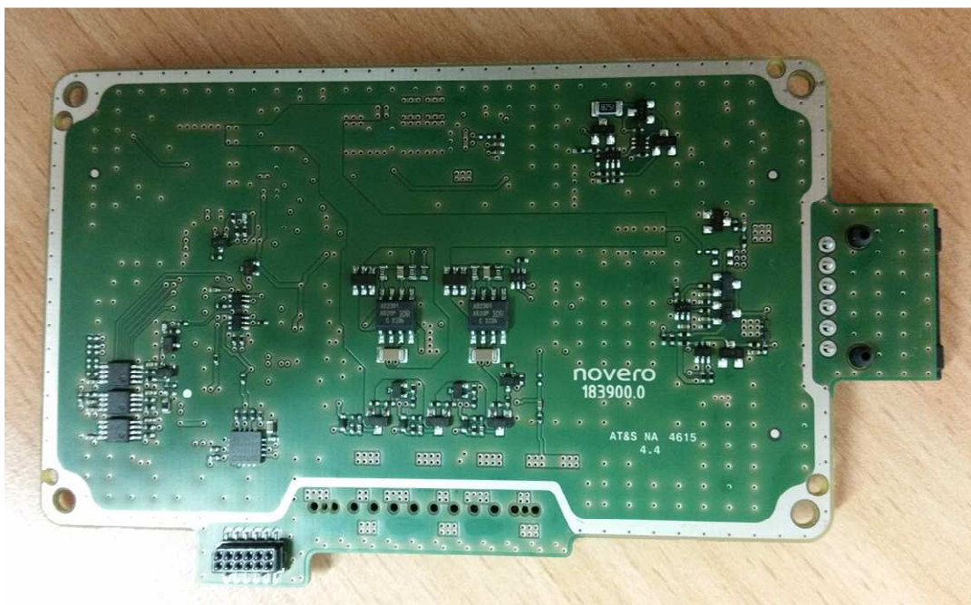
Bottom View Main board
