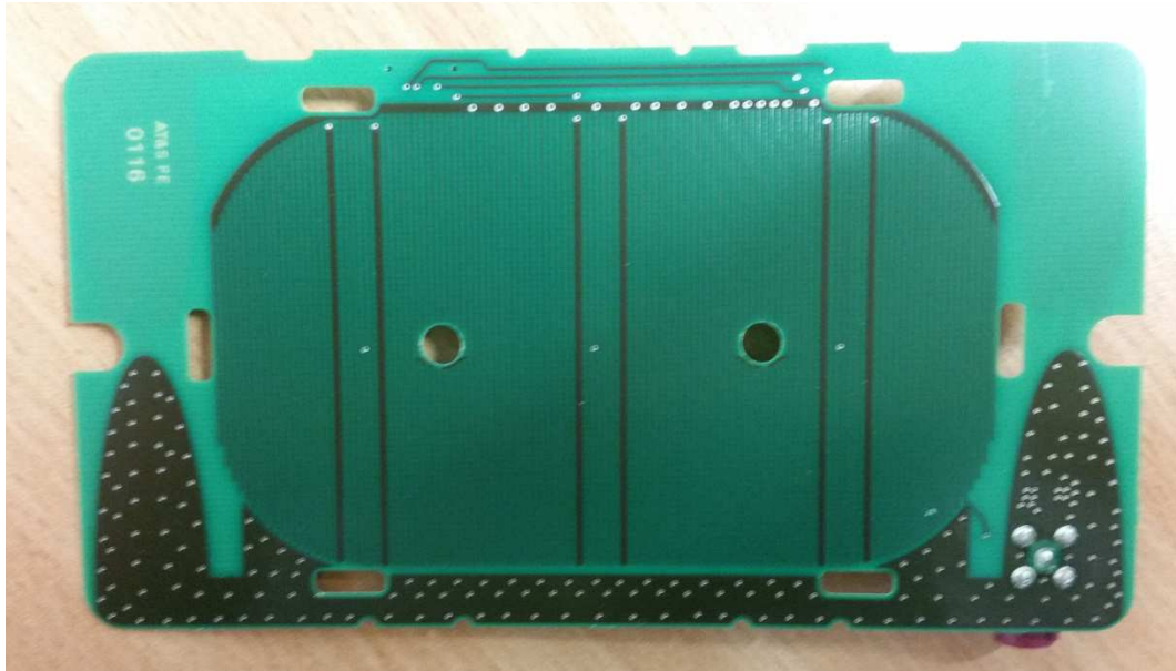
Bottom view antenna board
