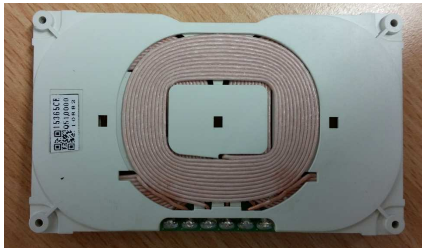
Top view 3 coil module with 1 coil
