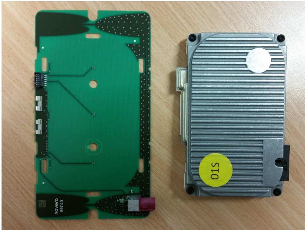
Antenna Board with coil module, main board and cooling element (mounted)
