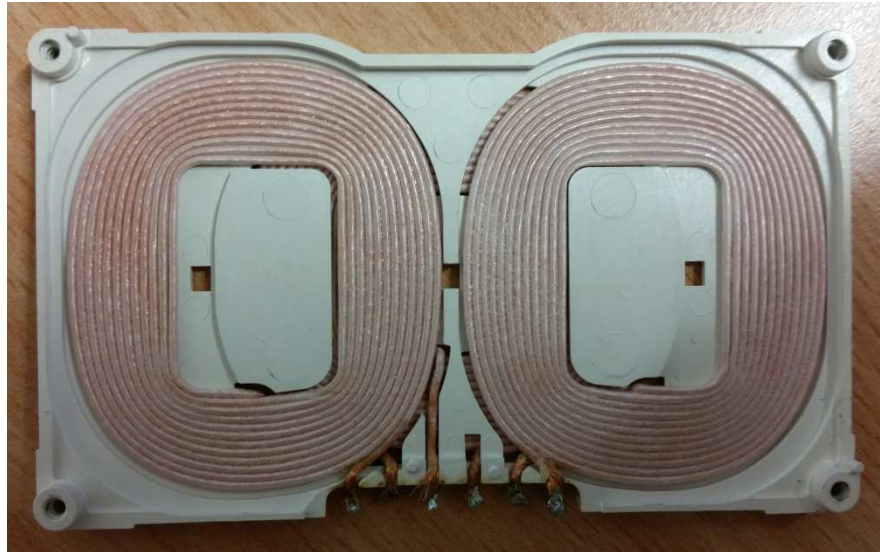
Inner view coil module with 2 coils
