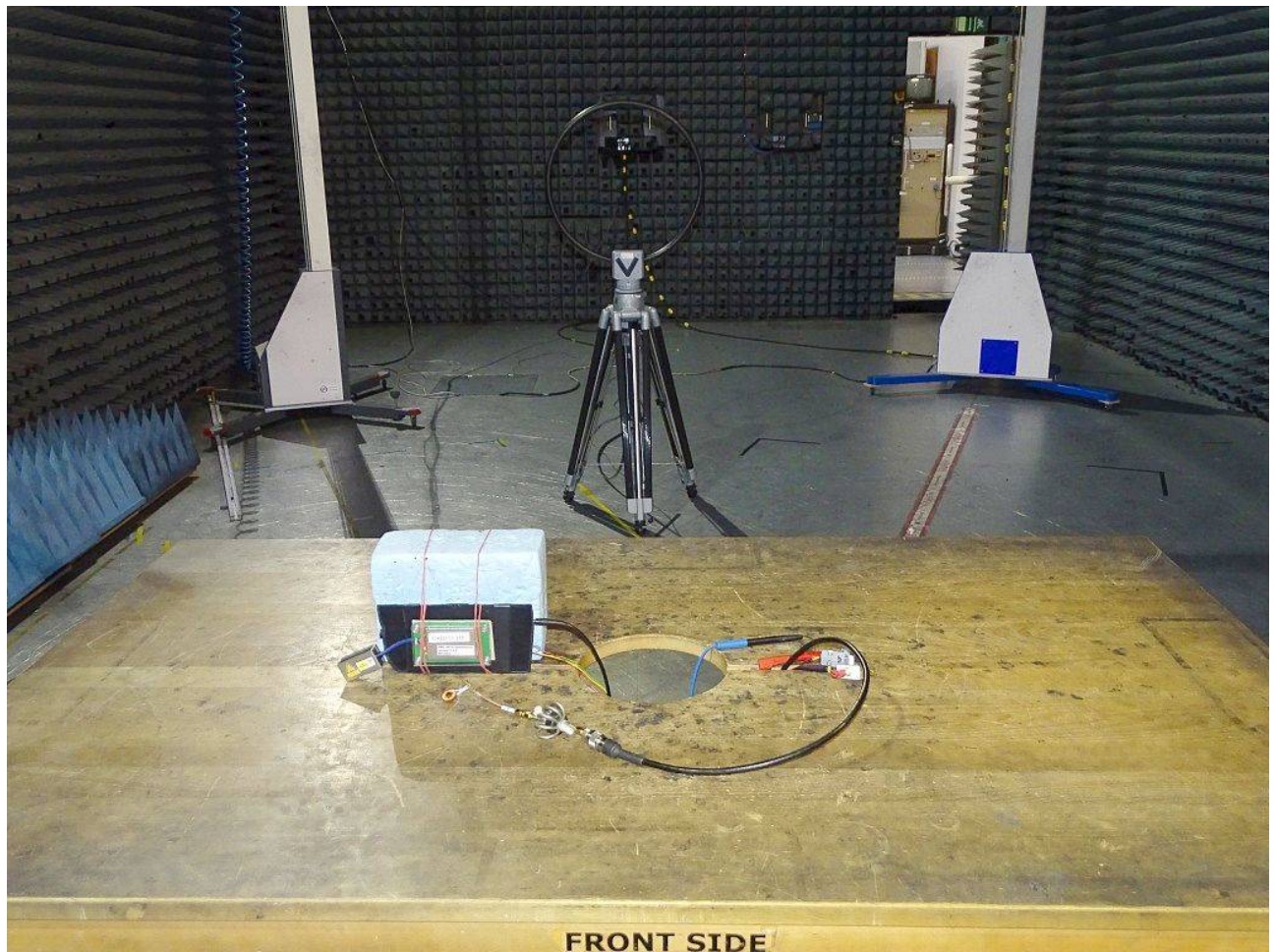
Photo 1: Test setup for radiated measurements (Enclosure, below 30 MHz, intentional radiator §15.209, ANSI C63.10) vertical EUT position is shown
