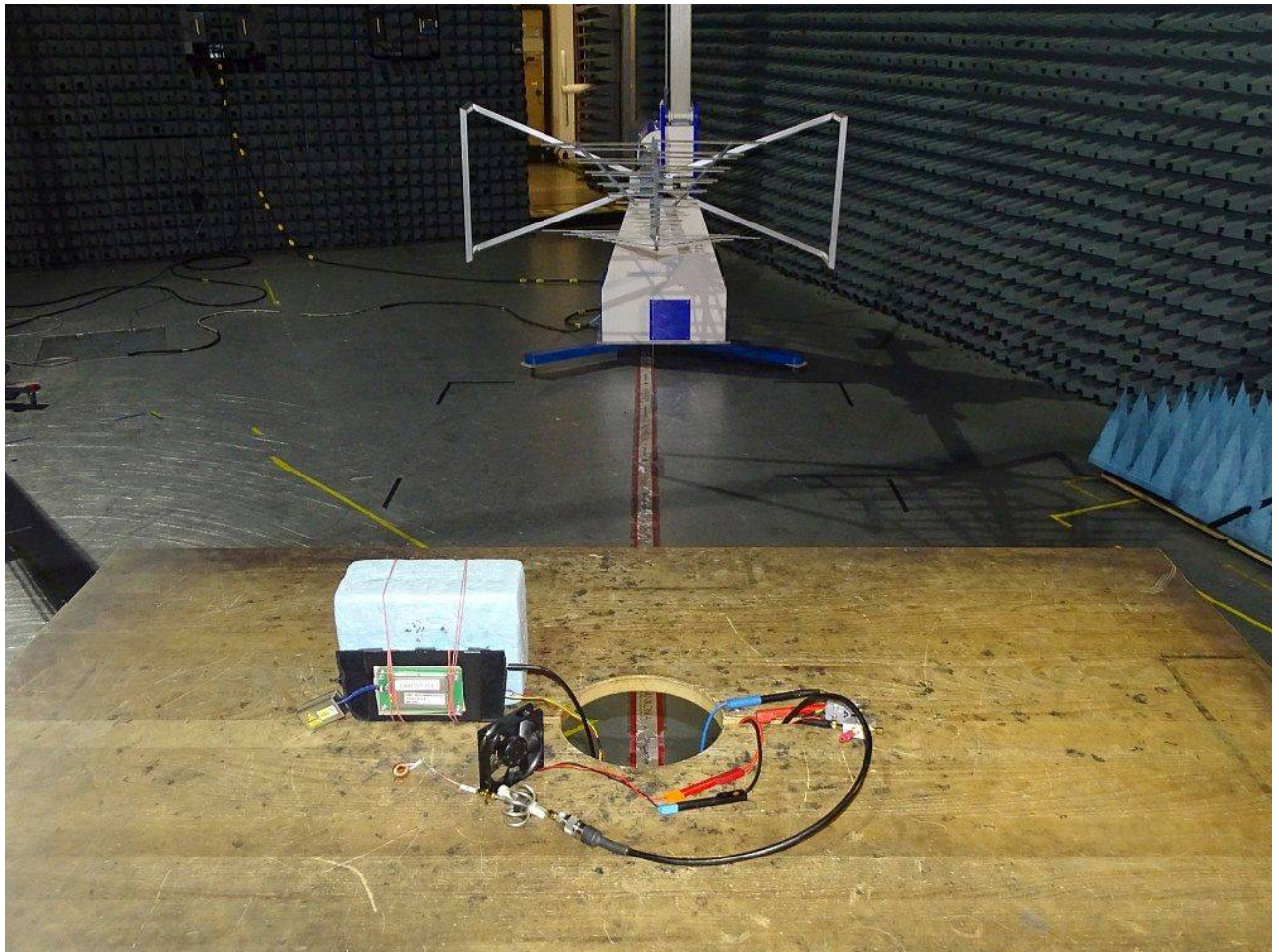
Photo 2: Test setup for radiated measurements (Enclosure, semi-anechoic chamber, 30 MHz to 1 GHz, intentional radiator §15, ANSI C63.10 vertical EUT position is shown
