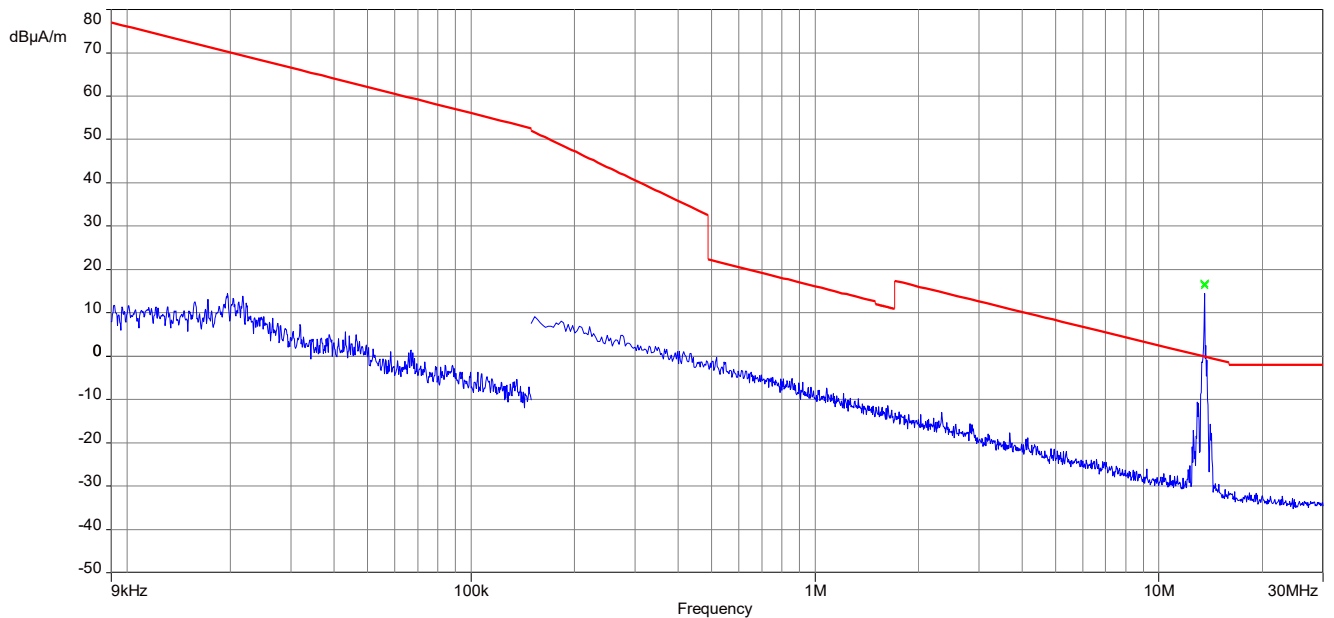
Plot 2: 9 kHz – 30 MHz, magnetic emissions ISED
