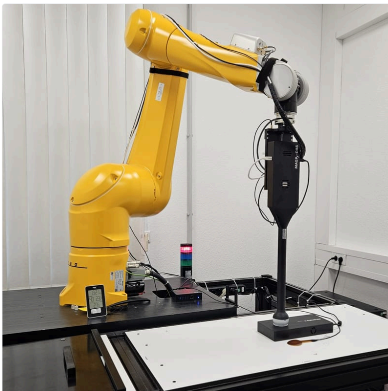
Photo 1 DASY8 WPT System
