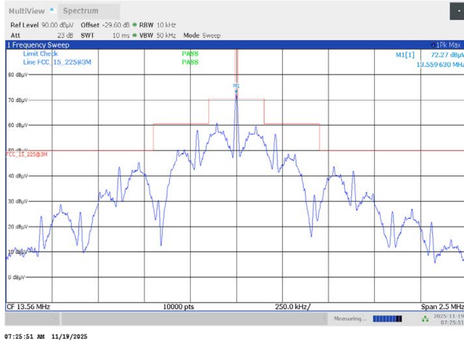
Plot 3: Spectrum mask (the limits are recalculated according to the ANSI C63.10 sub clause 6.4)
