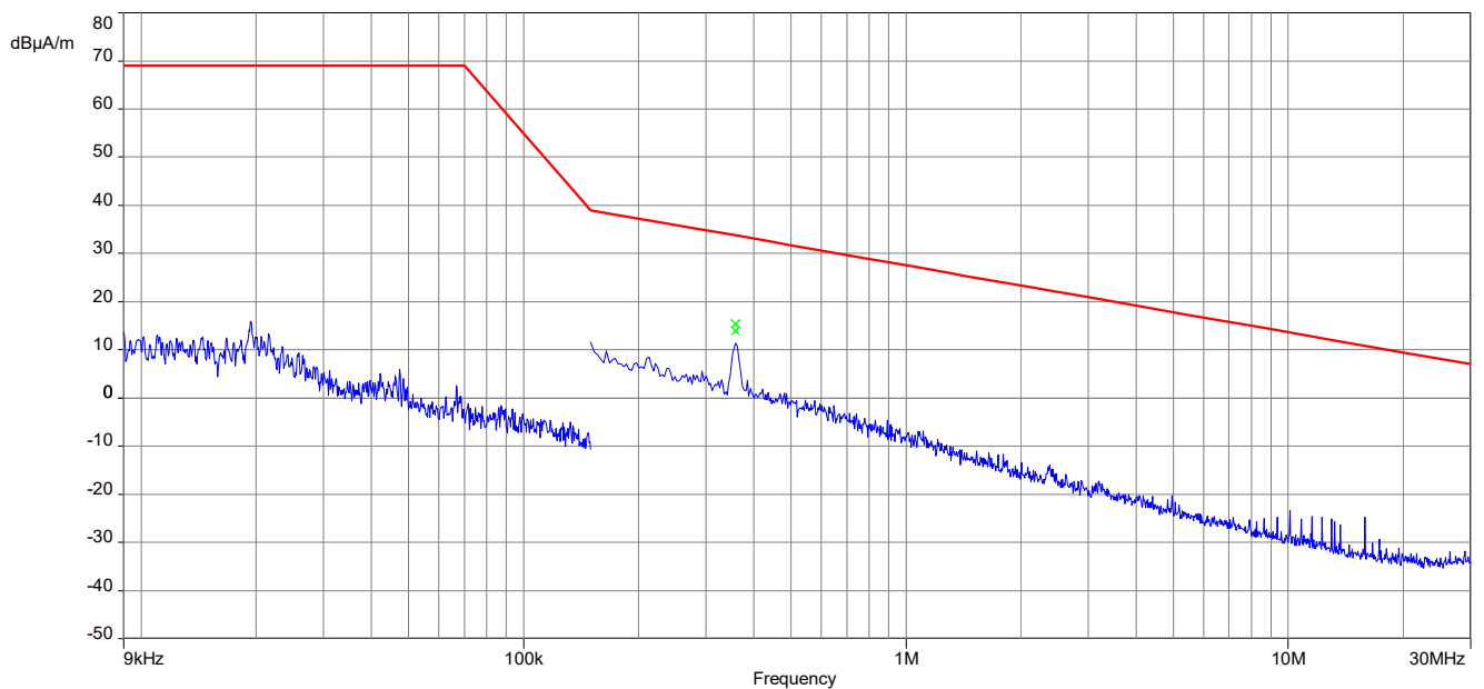
Plot 12: 9 kHz – 30 MHz, magnetic spurious emissions ISSED, 360 kHz
