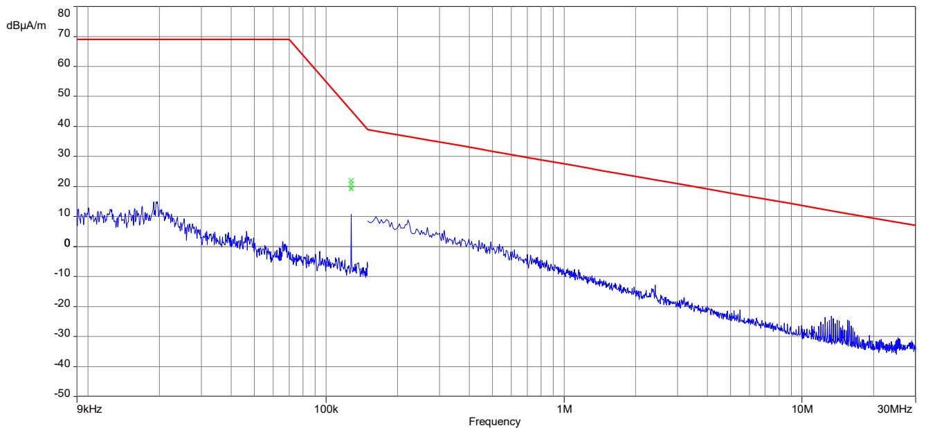
Plot 10: 9 kHz – 30 MHz, magnetic spurious emissions ISSED, 129.75 kHz charging mode
