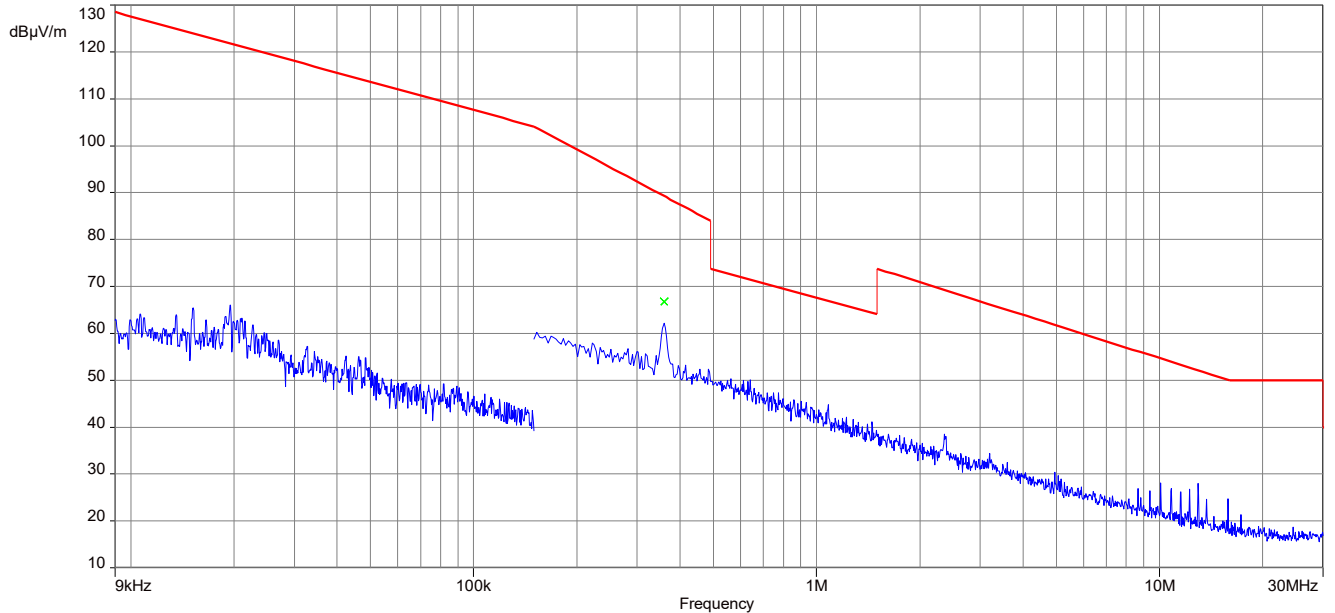
Plot 11: 9 kHz – 30 MHz, magnetic spurious emissions FCC, 360 kHz
