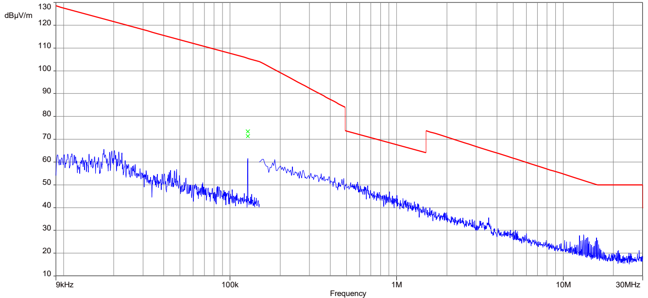
Plot 3: 9 kHz – 30 MHz, magnetic spurious emissions FCC, 126.55 kHz charging mode
