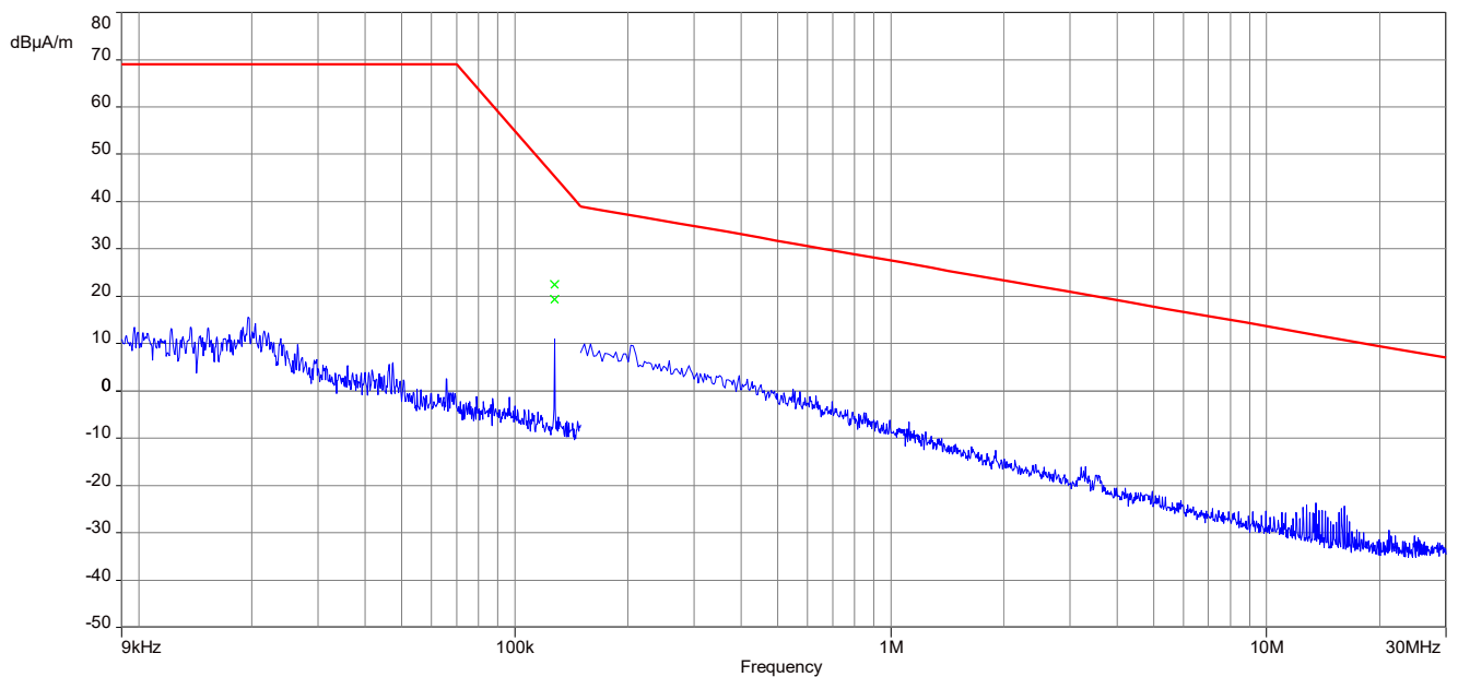
Plot 2: 9 kHz – 30 MHz, magnetic spurious emissions ISSED, 125.35 kHz charging mode
