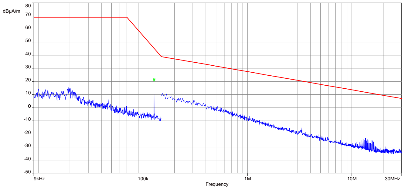
Plot 4: 9 kHz – 30 MHz, magnetic spurious emissions ISSED, 126.55 kHz charging mode
