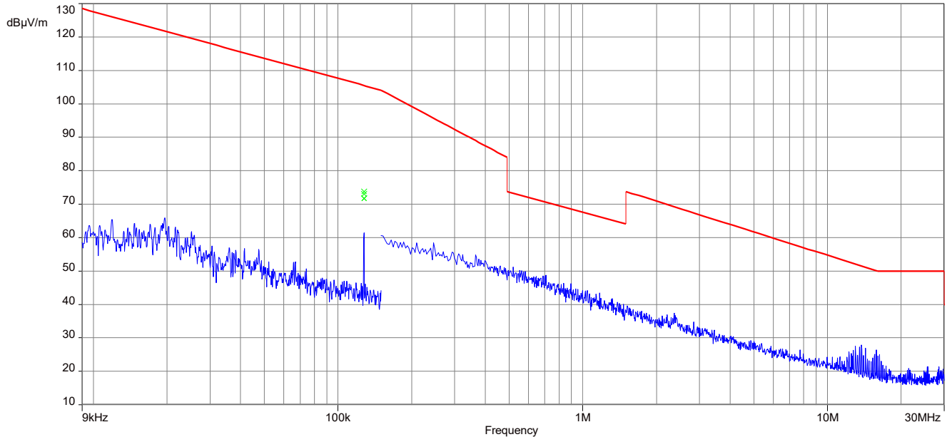
Plot 7: 9 kHz – 30 MHz, magnetic spurious emissions FCC, 128.55 kHz charging mode
