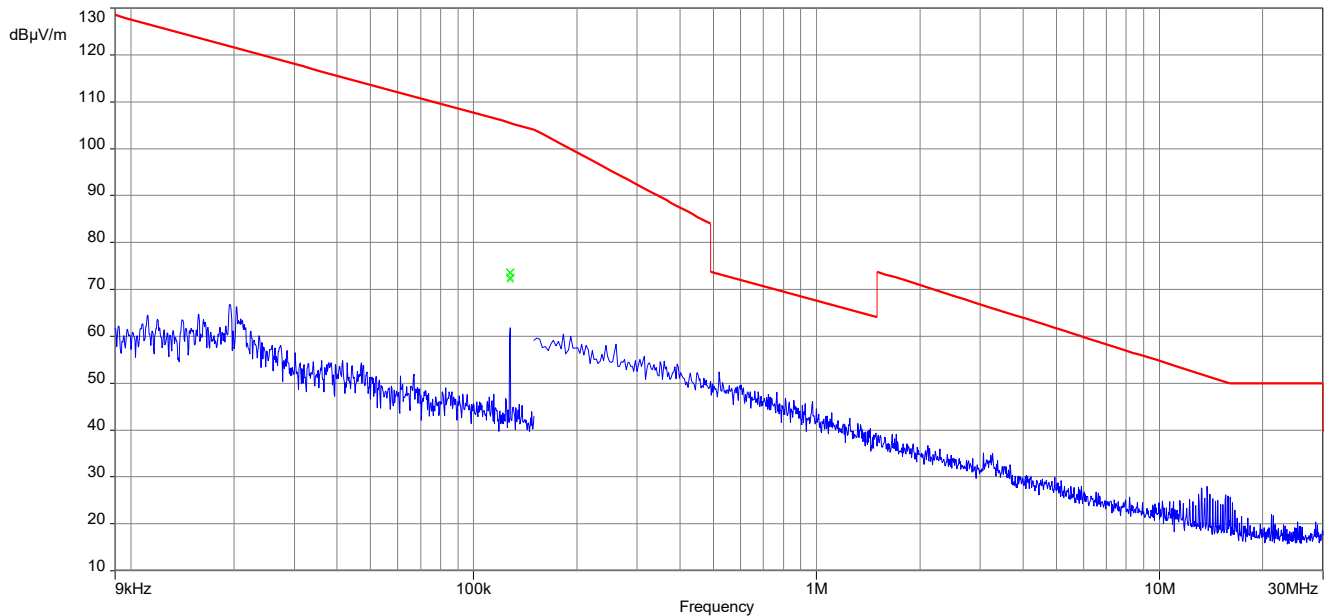
Plot 1: 9 kHz – 30 MHz, magnetic spurious emissions FCC, 125.35 kHz charging mode
