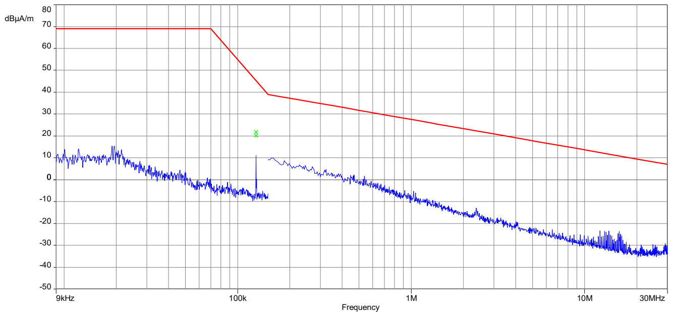
Plot 8: 9 kHz – 30 MHz, magnetic spurious emissions ISSED, 128.55 kHz charging mode
