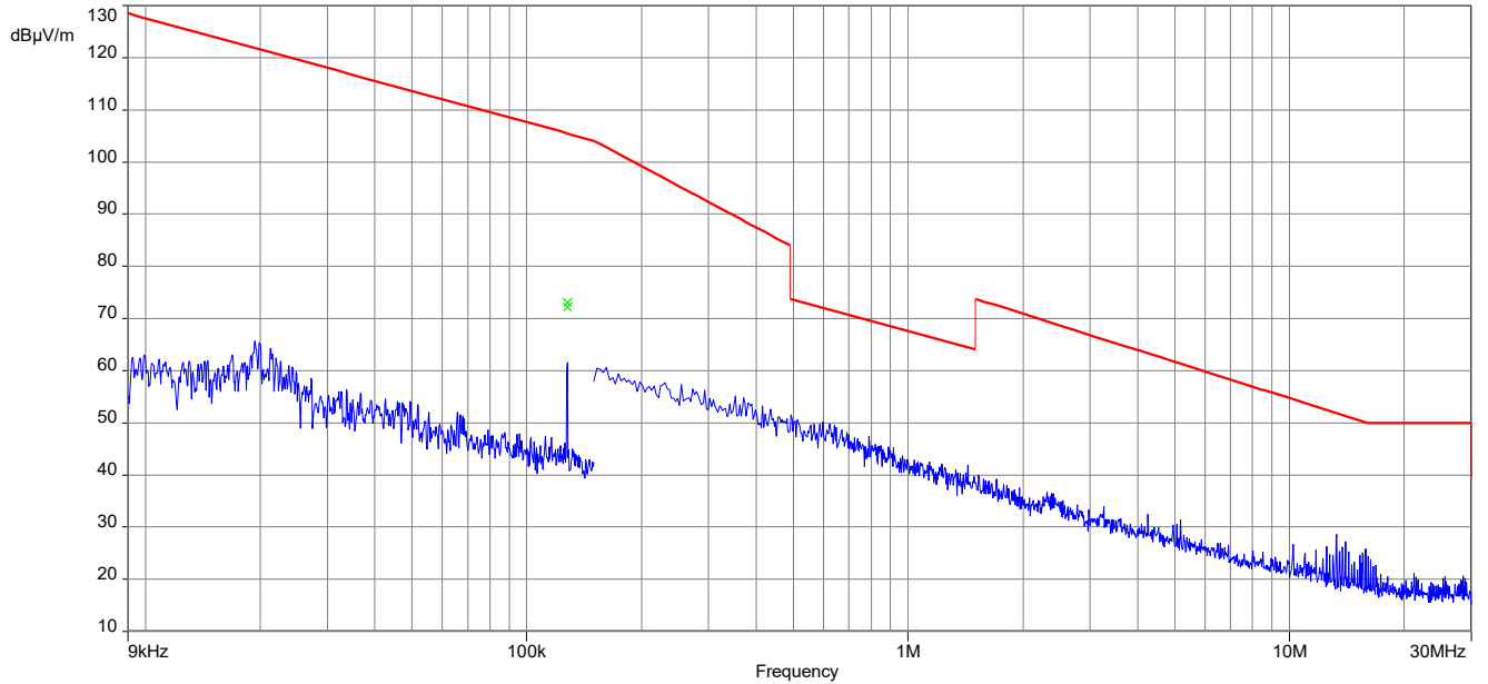
Plot 5: 9 kHz – 30 MHz, magnetic spurious emissions FCC, 127.55 kHz charging mode
