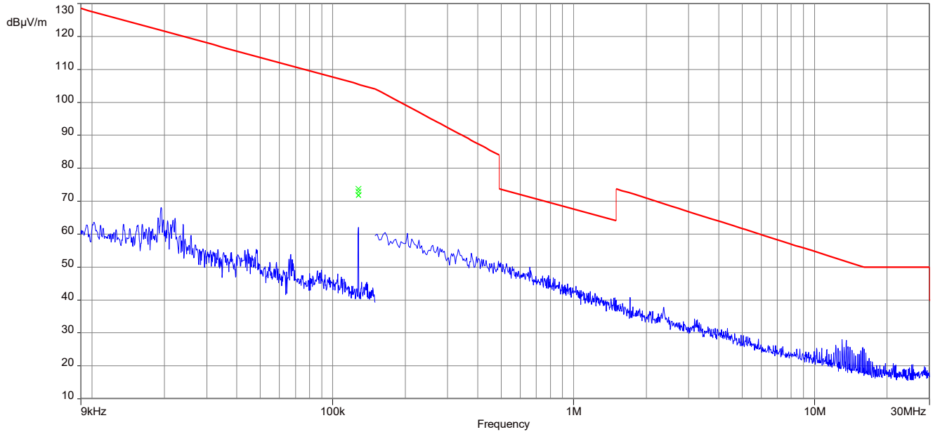
Plot 9: 9 kHz – 30 MHz, magnetic spurious emissions FCC, 129.75 kHz charging mode
