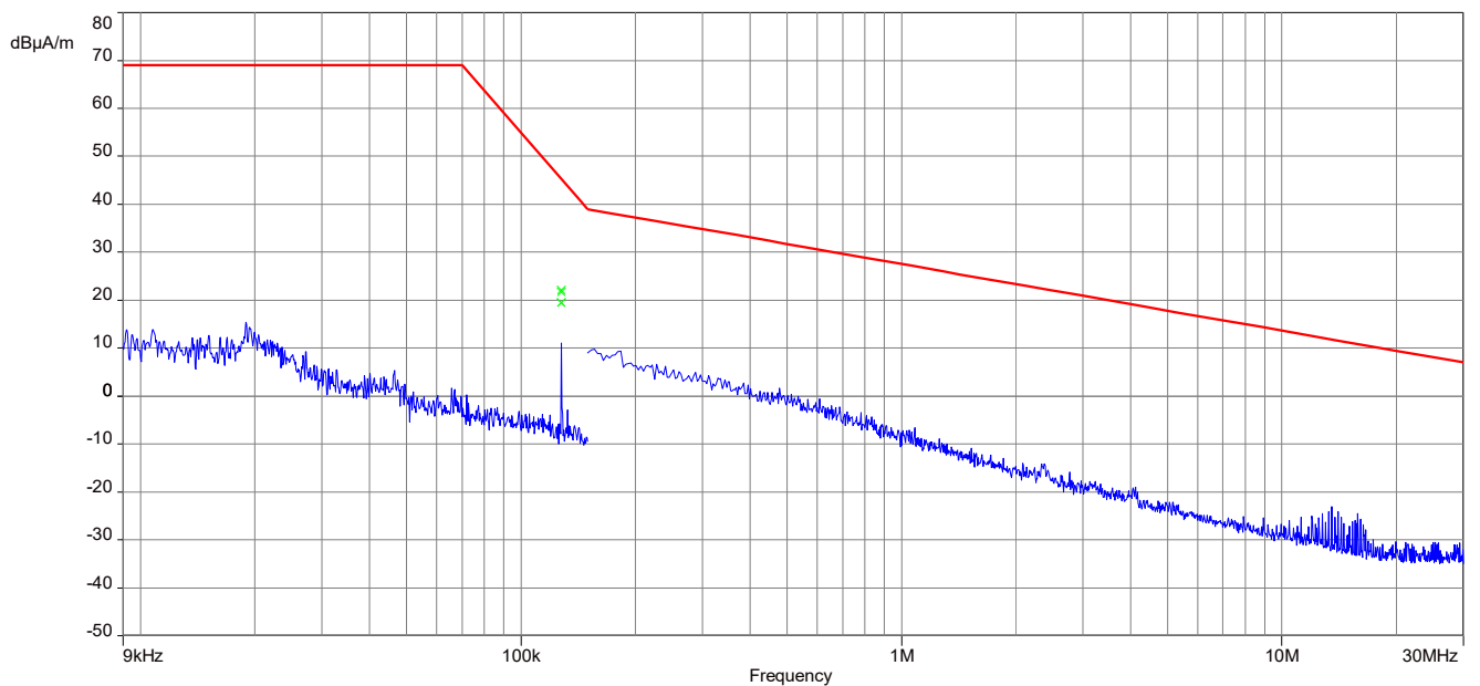
Plot 6: 9 kHz – 30 MHz, magnetic spurious emissions ISED, 127.55 kHz charging mode
