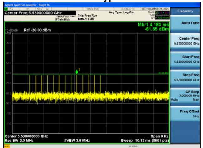
Radars type 4
