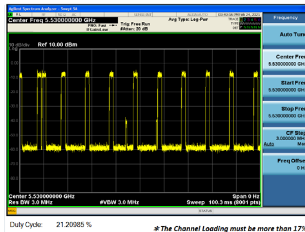
WLAN traffic
