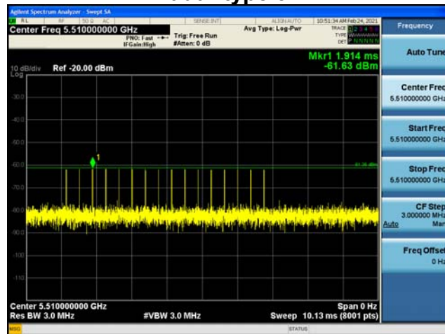
Radar type 4
