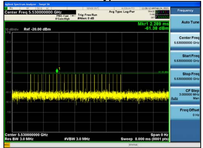
Radars type 3
