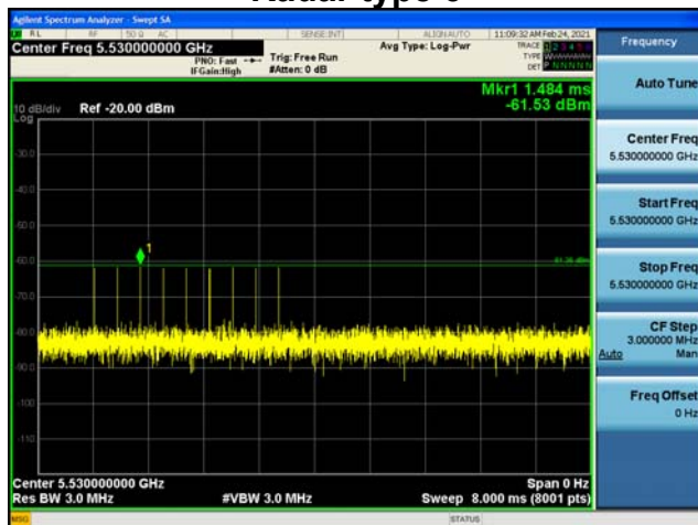
Radar type 6
