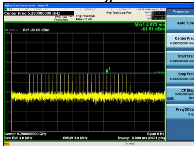
Radars type 3
