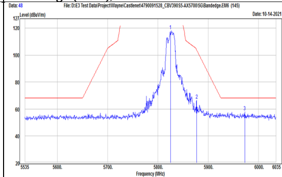
TX, 802.11a (Ch 165) Band Edge (Peak), Vertical
