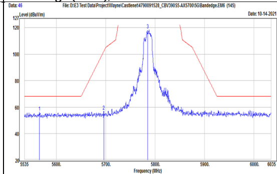
TX, 802.11a (Ch 157) Band Edge (Peak), Vertical
