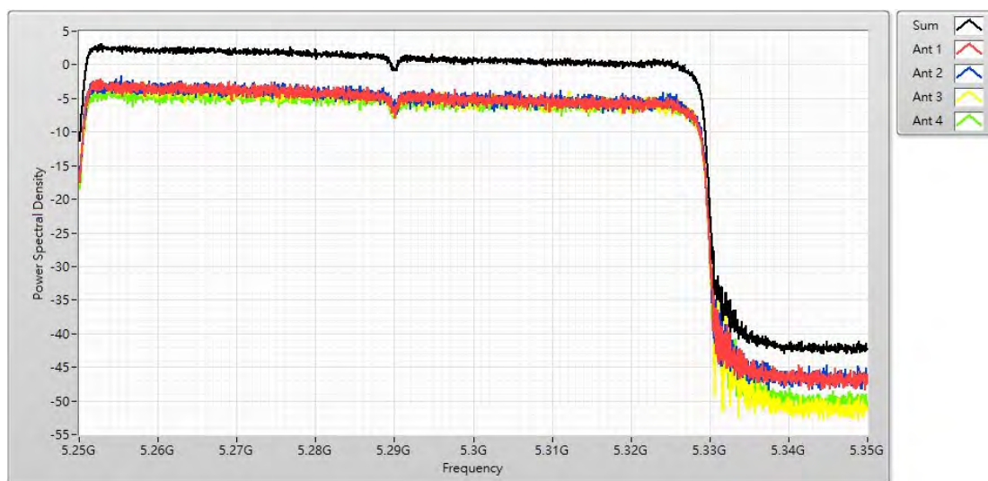
Channel 50 (5250MHz (Band 1))
