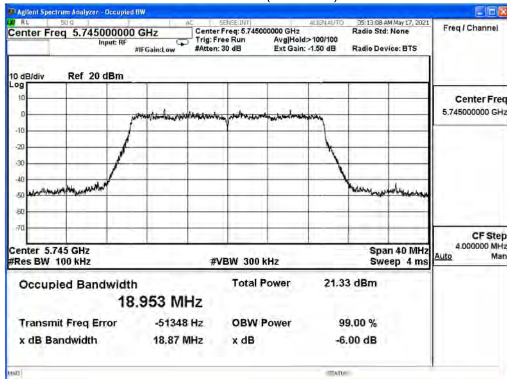
Channel 149 (5745MHz)
