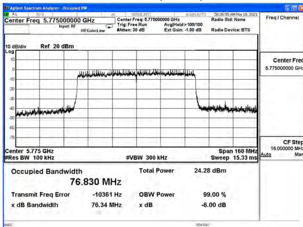
Channel 155 (5775MHz)
