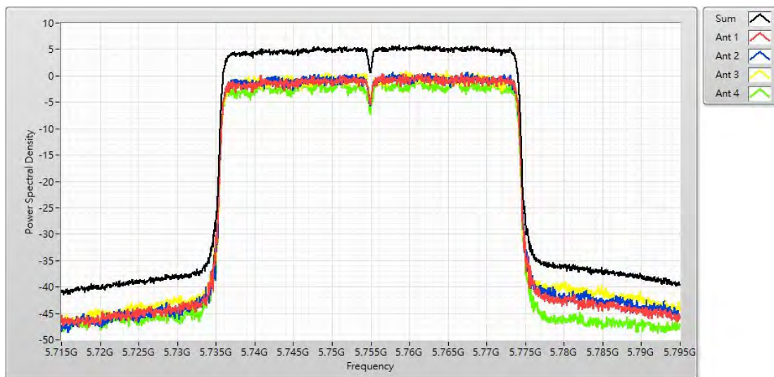
Channel 151 (5755MHz)
