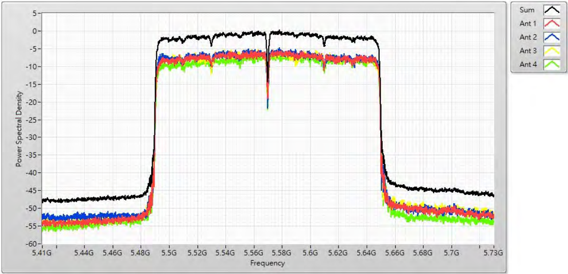
Channel 114 (5570MHz)
