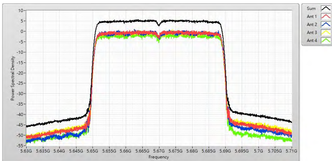
Channel 134 (5670MHz)
