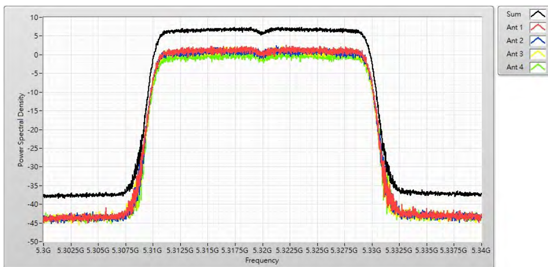
Channel 64 (5320MHz)
