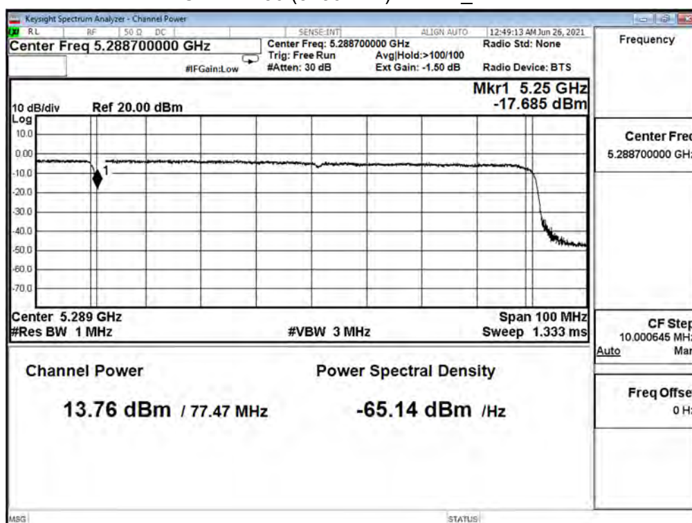
Channel 50 (5250MHz) Band 2_Ant. 1
