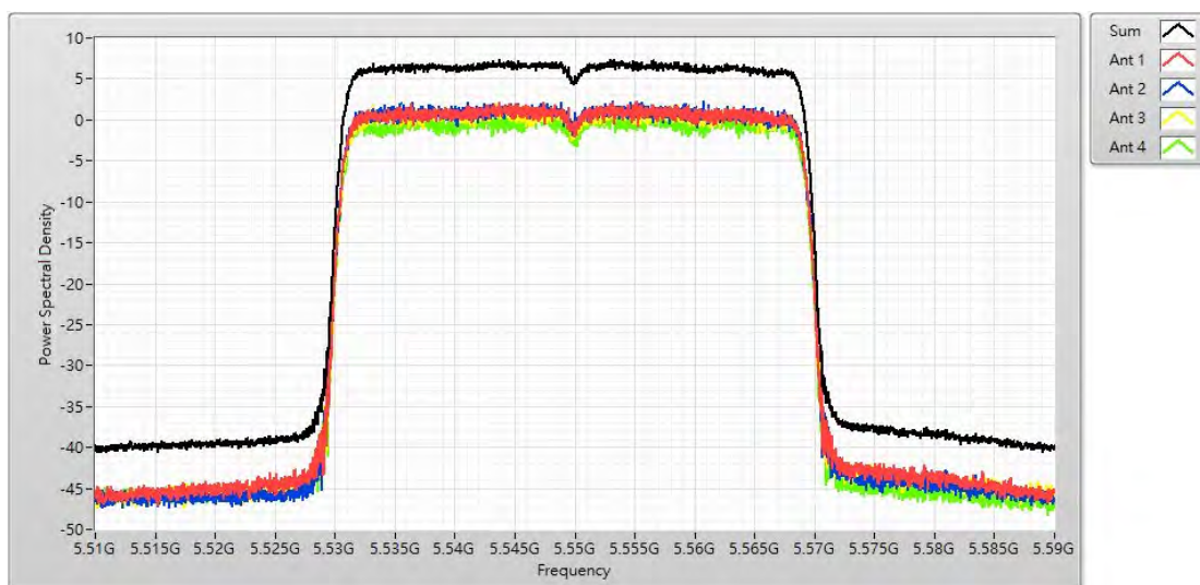
Channel 110 (5550MHz)
