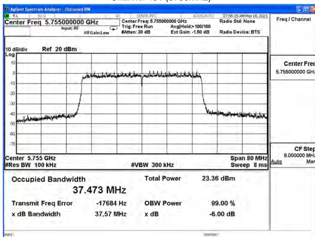
Channel 151 (5755MHz)
