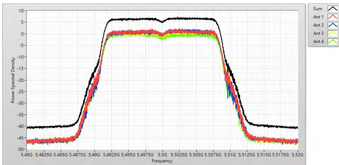
Channel 100 (5500MHz)
