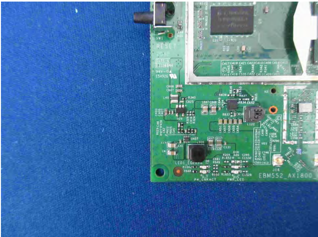
(42) EUT Photo
