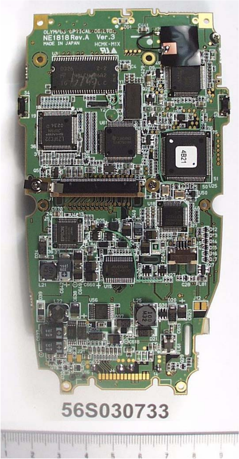
EUT PCB View 2
