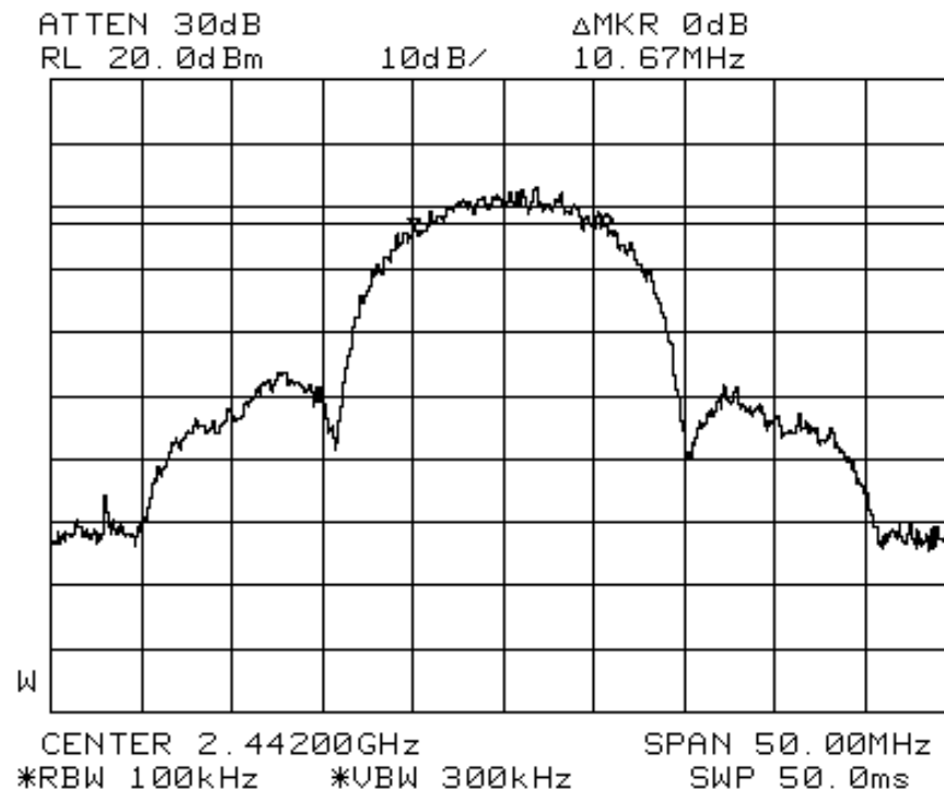
Plot 33 – Channel 7 @ 802.11b 5.5Mbps
