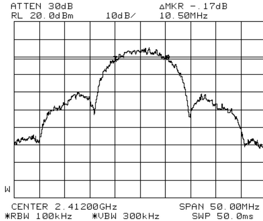
Plot 32 – Channel 1 @ 802.11b 5.5Mbps
