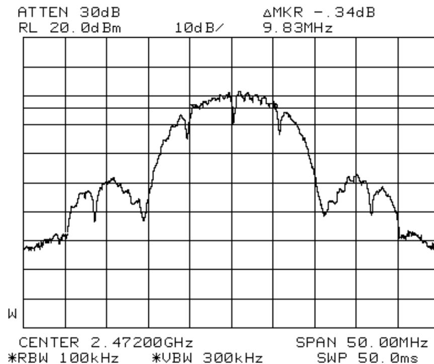
Plot 31 - Channel 13 @ 802.11b 2Mbps
