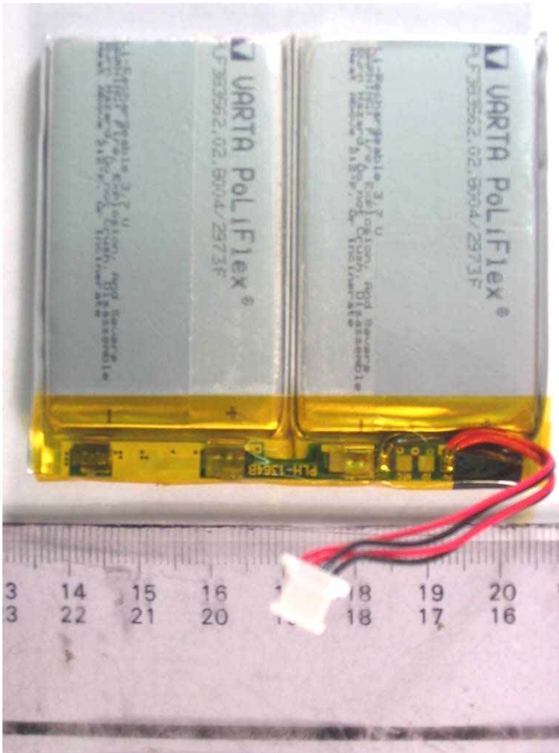
EUT Rechargeable Battery Pack Front View
