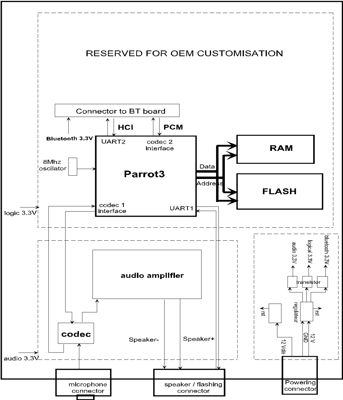
Block_diagram CK3000 Main_board
