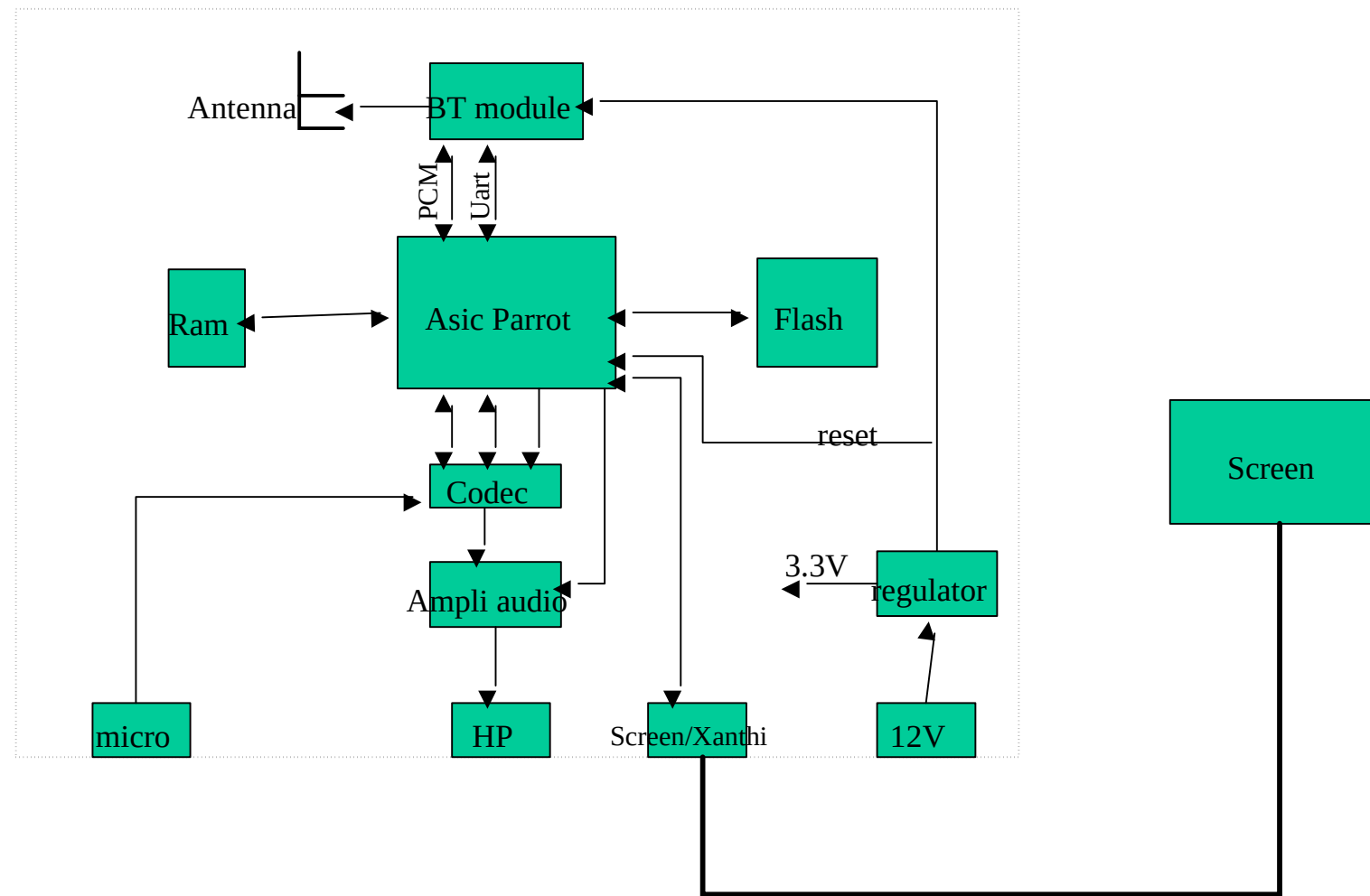
Block Diagram CK3100
