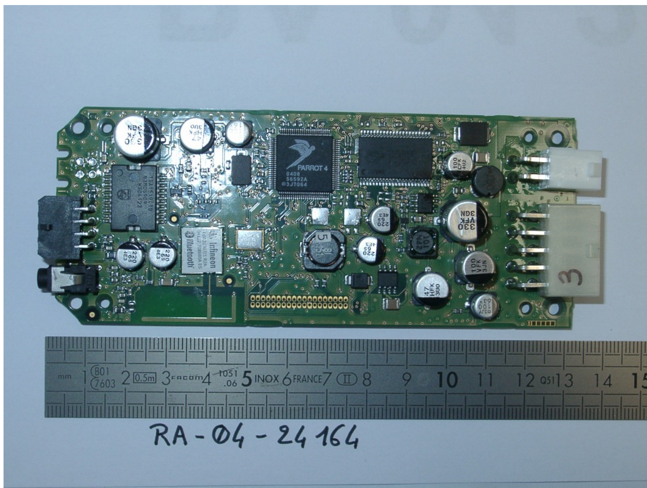
Printed circuit board: face 1
