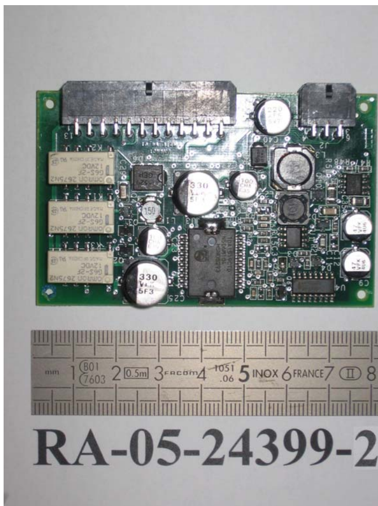
Printed circuit board MUTE: face 1
