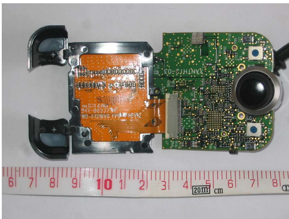
Printed circuit board XANTHI2: face 2
