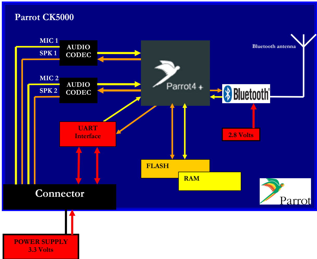
CK5000 Simplified Block Diagram
