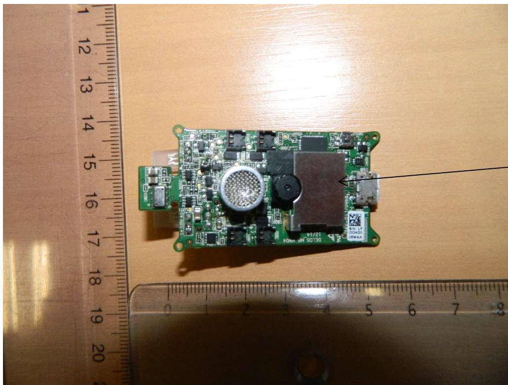
Board (Bottom)
