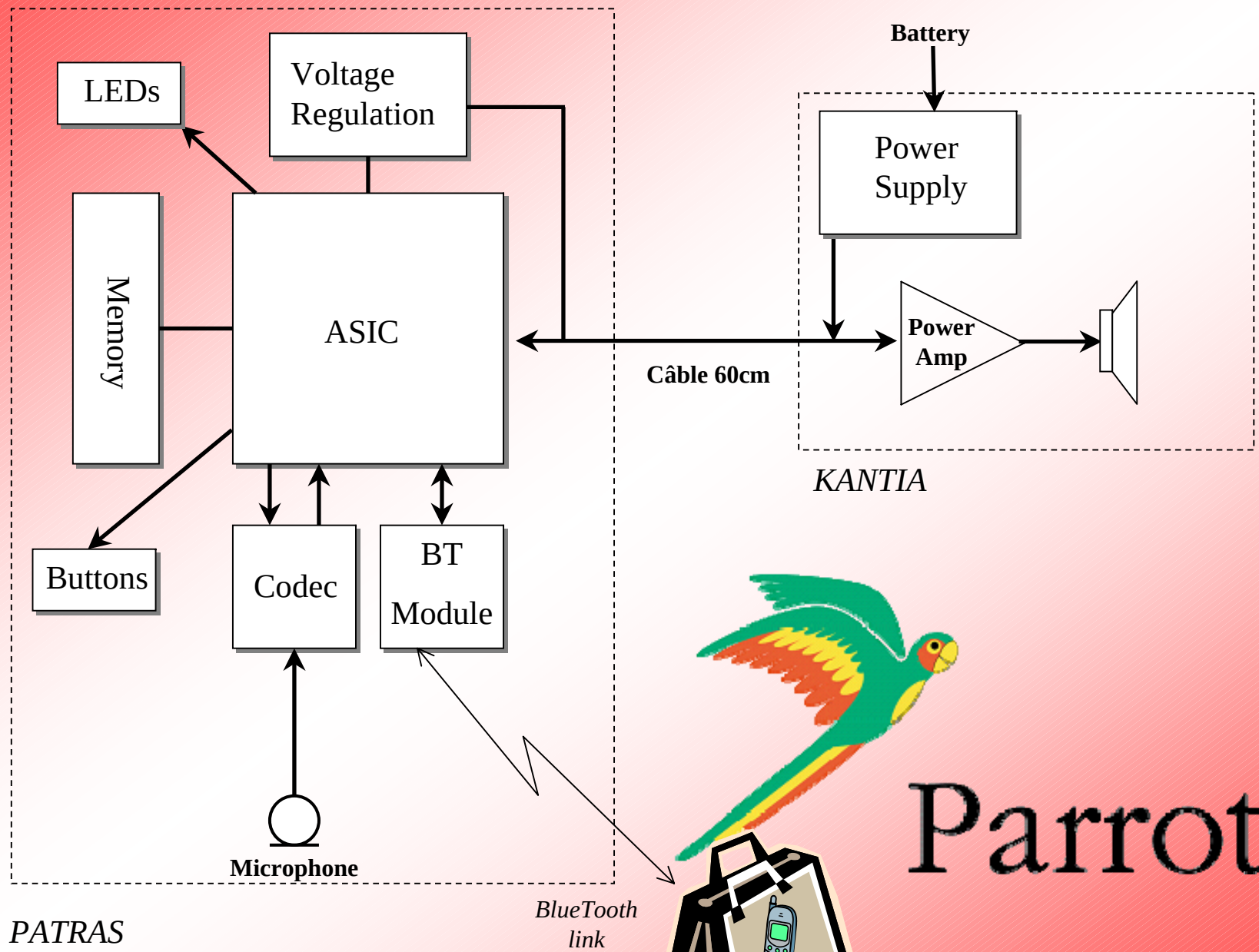
Easydrive : Block diagram
